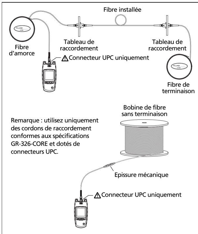
Figure 7. Raccordements
