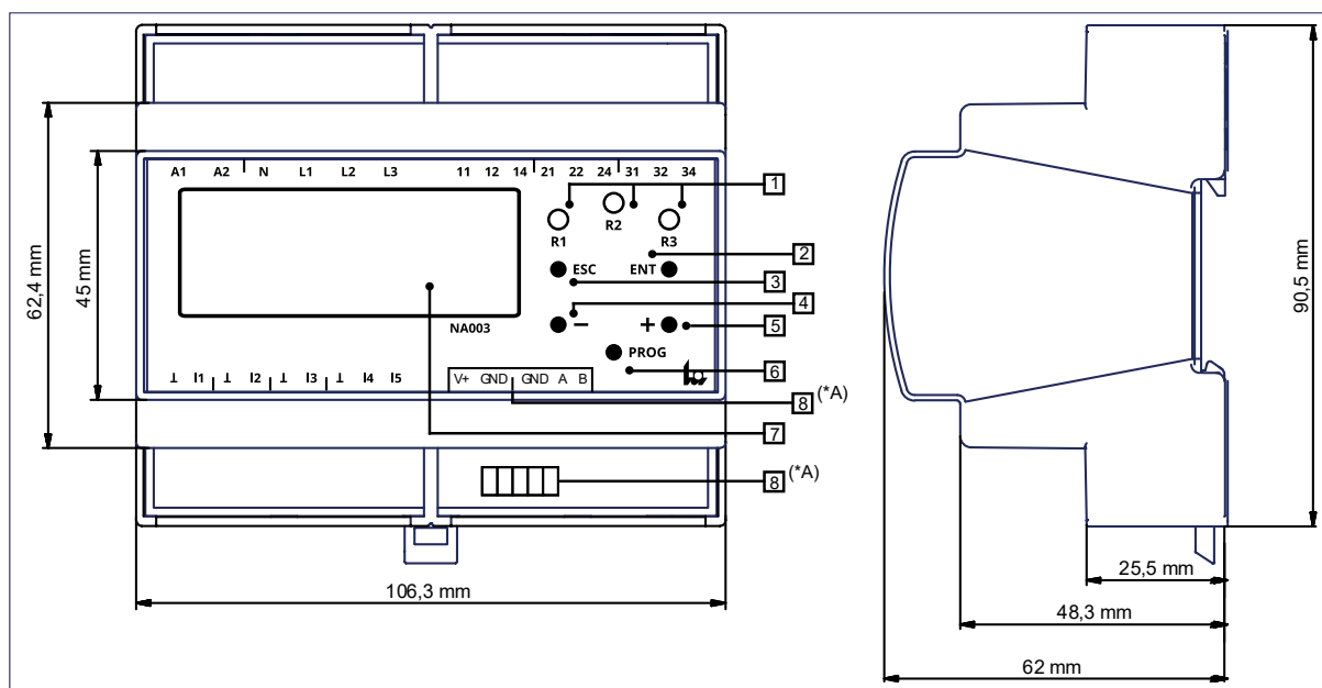
Figure 1: NA003.COM(*A) Key notes and dimensions
