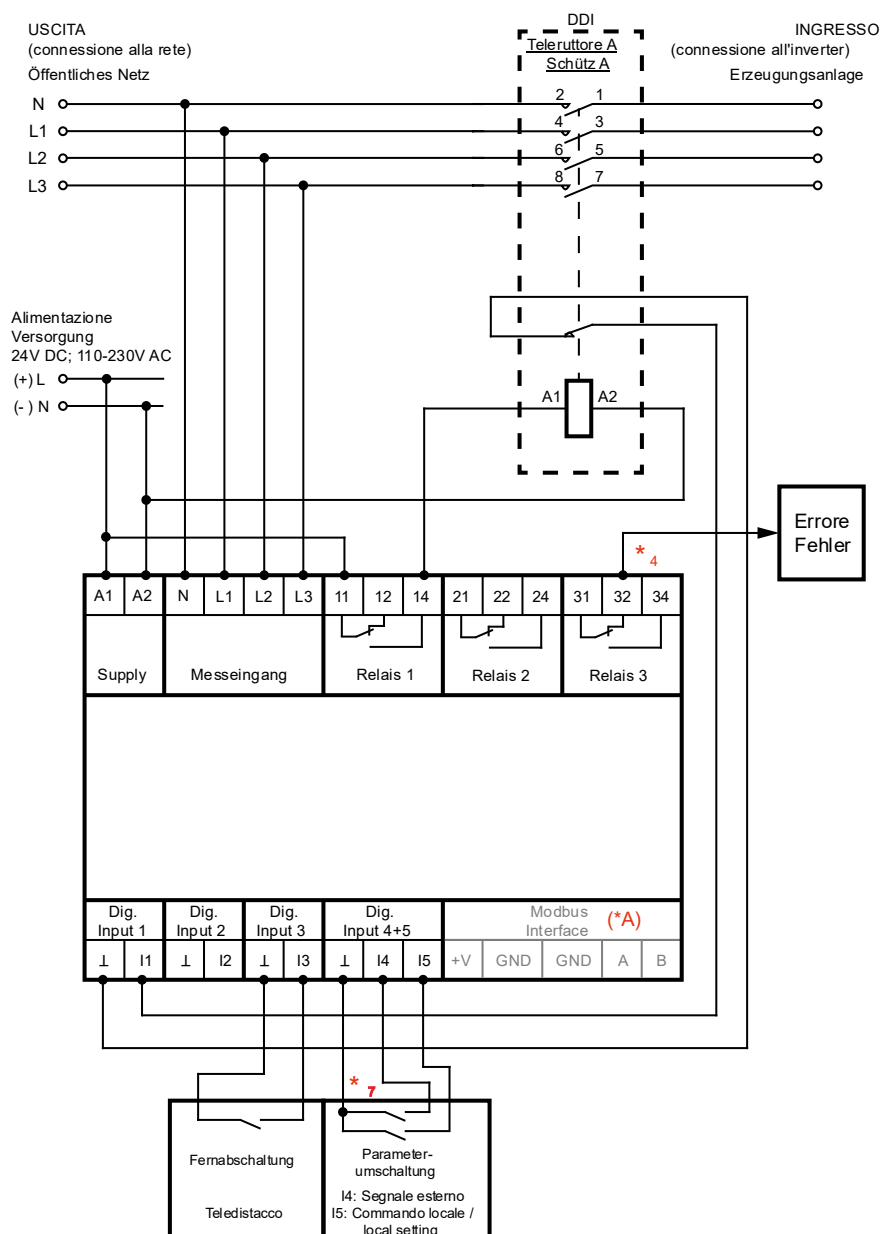
Figure 4: Circuit diagram 3 (CEI 0-21)
