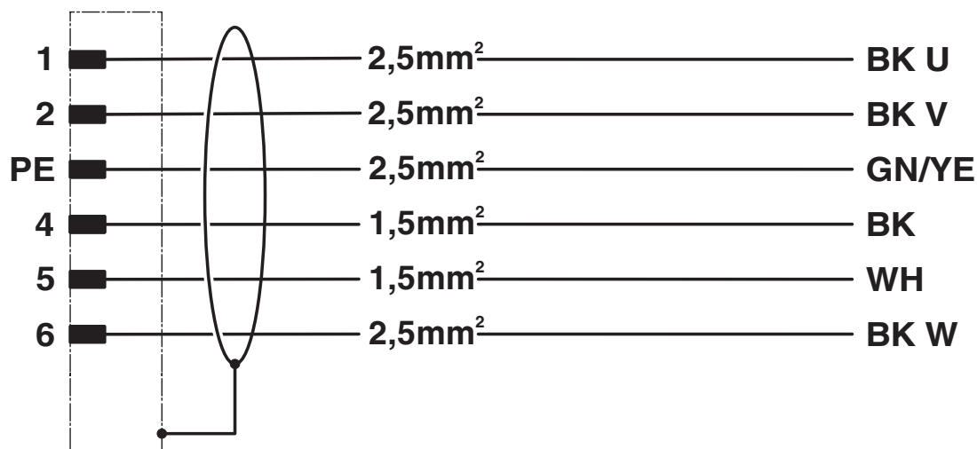
Circuit diagram
