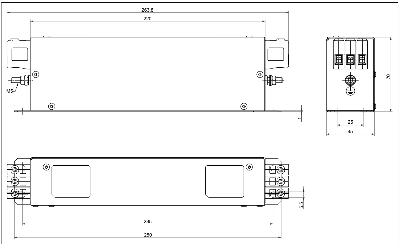
Figure 1: Dimension diagram and installation dimensions
