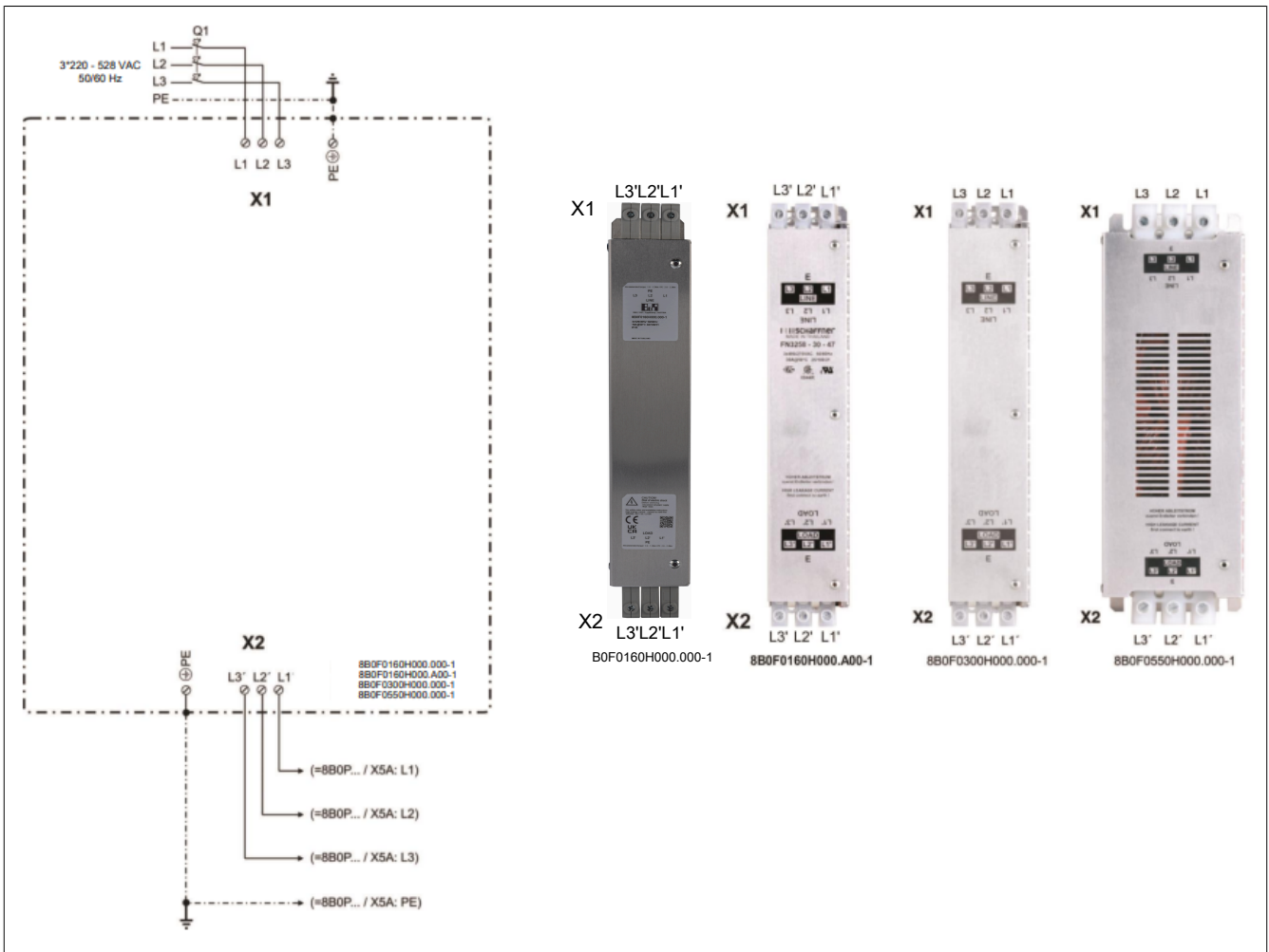
Figure 2: 8B0F0160H000.A00-1, 8B0F0300H000.000-1, 8B0F0550H000.000-1, 8B0F0160H000.000-1 - Pinout overview
