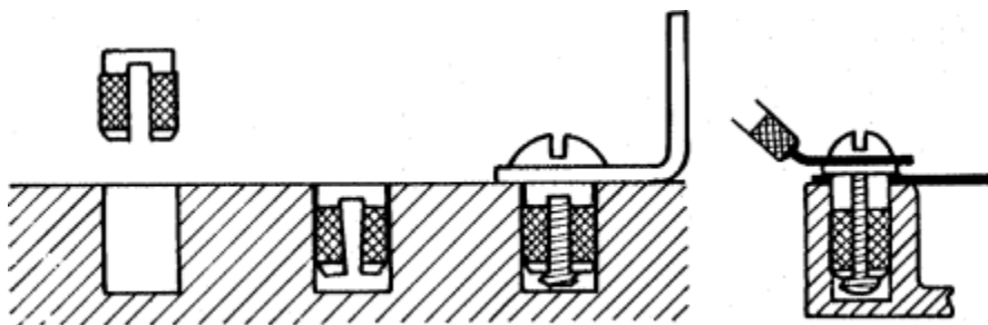
INSERTION METHOD AND TYPICAL APPLICATIONS
