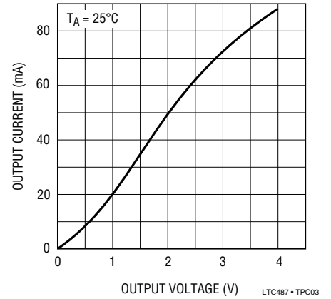
Driver Output Low Voltage vs Output Current
