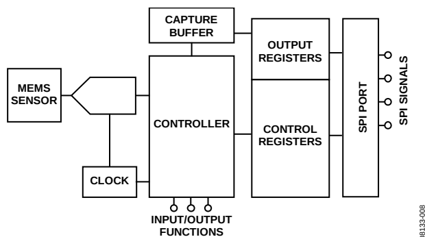
Figure 12. Simplified Sensor Signal Processing Diagram
