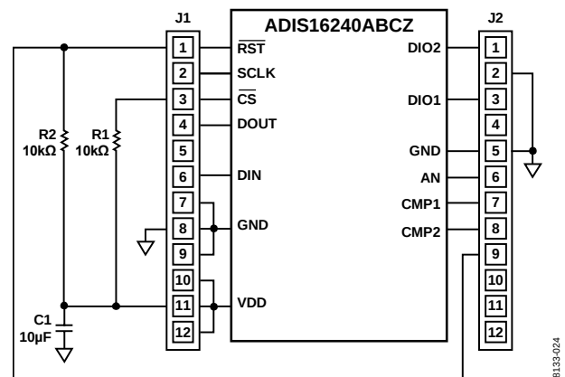
Figure 25. Electrical Schematic
