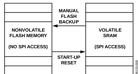
Figure 13. Control Registers—SRAM and Flash Memory Diagram
