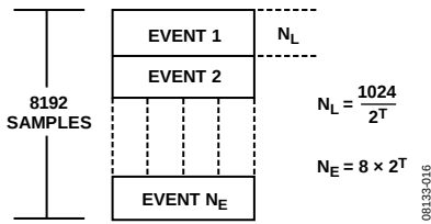
Figure 20. Event Storage in Buffer Memory
