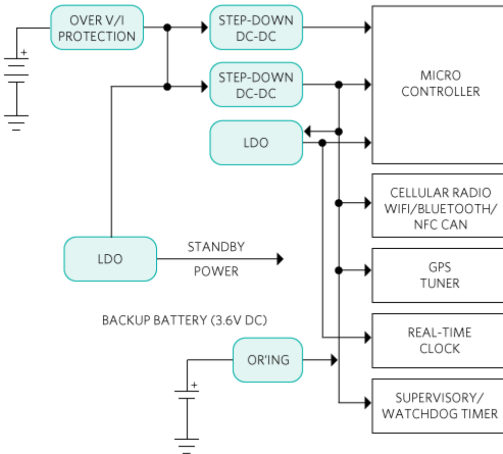
Figure 2. Typical fleet tracking/management power architecture.
