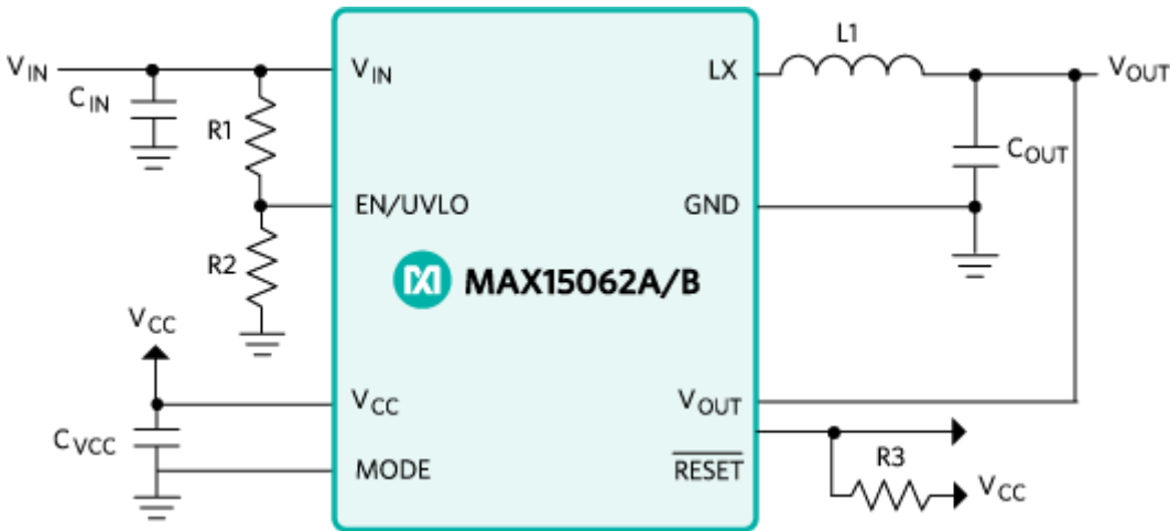
Figure 7. MAX15062A (3.3V V_{OUT} )/MAX15062B (adjustable V_{OUT} ) typical application schematic.
