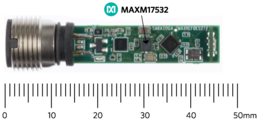
Figure 9. MAXM17532 power module in a tiny proximity sensor.
