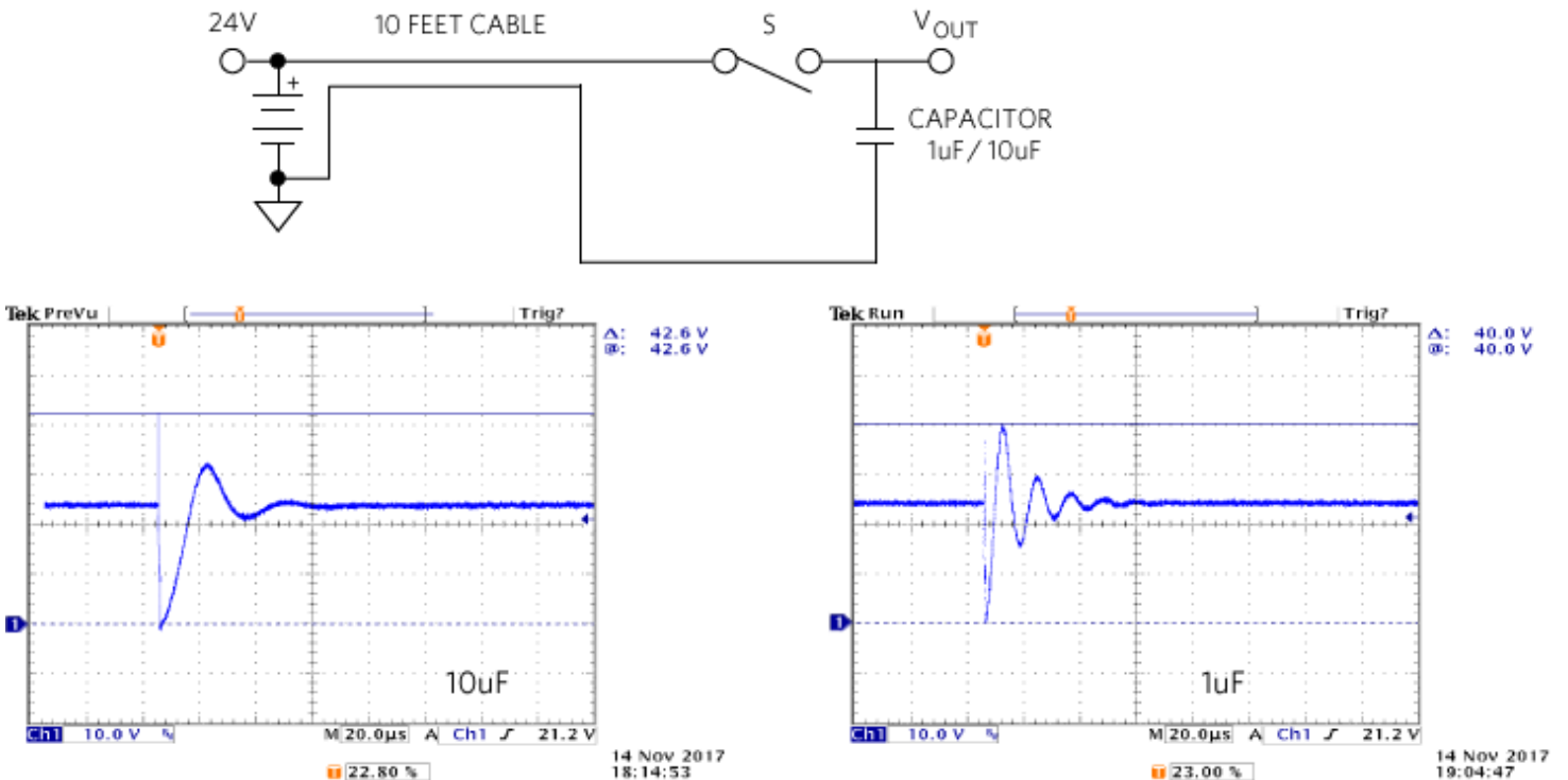
Figure 4. Cable ringing at initial plug-in.
