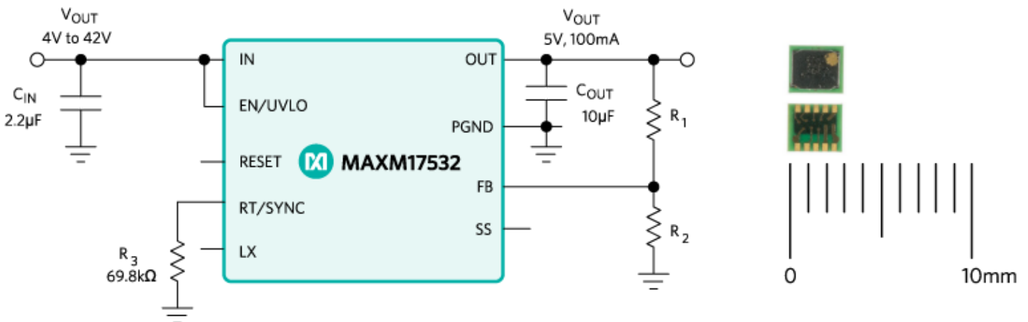
Figure 8. MAXM17532 typical application schematic.
