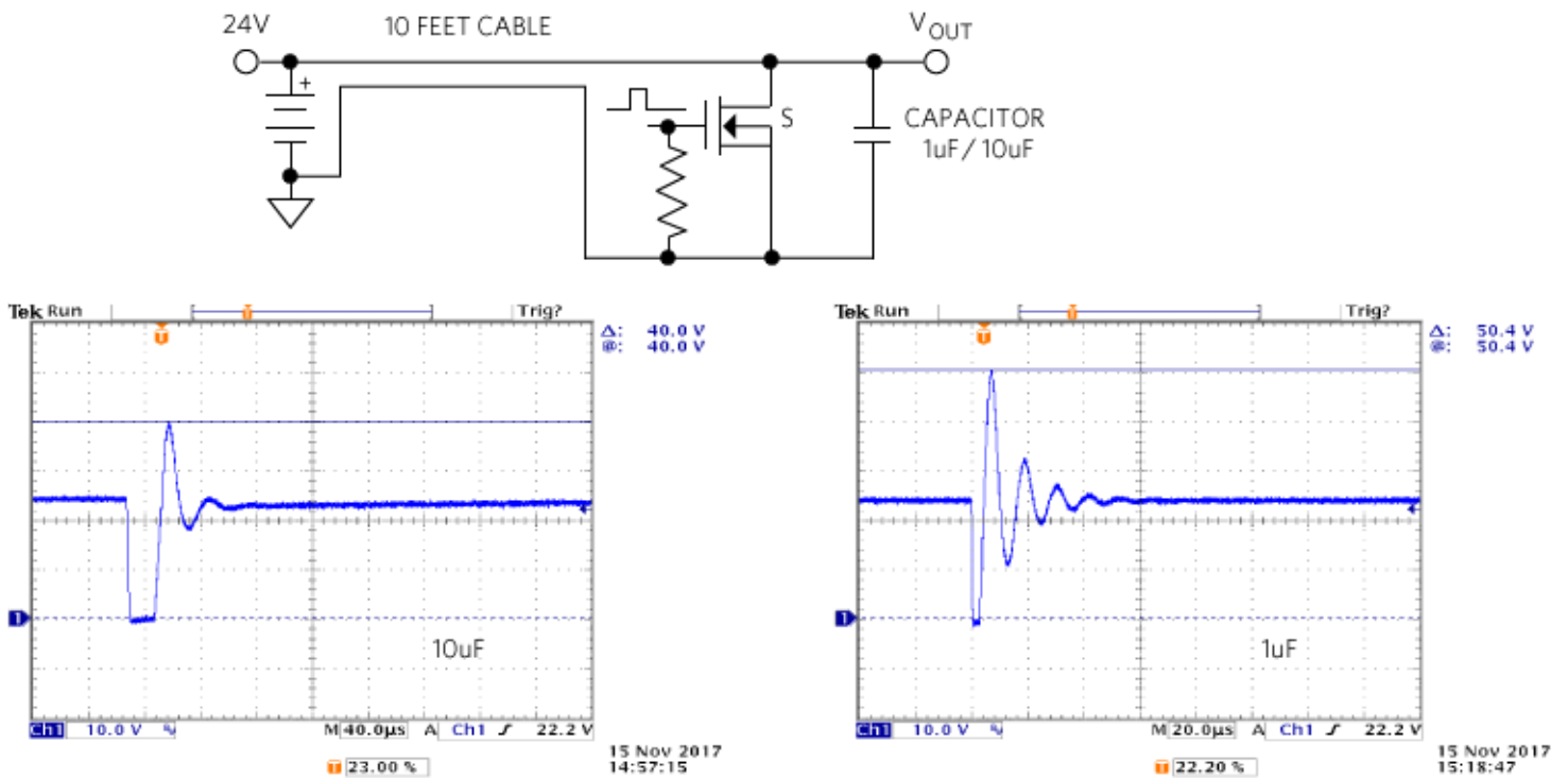
Figure 5. Cable ringing after a brief short-circuit condition.
