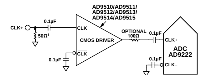
Figure 67. Single-Ended 3.3 V CMOS Sample Clock
