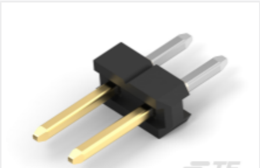
TE Part #2355181-2 2P,2MM,BRK HDR,SRVT,2.8,0.38AU, BOX
