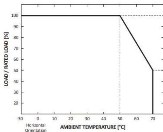
DERATING CURVE
