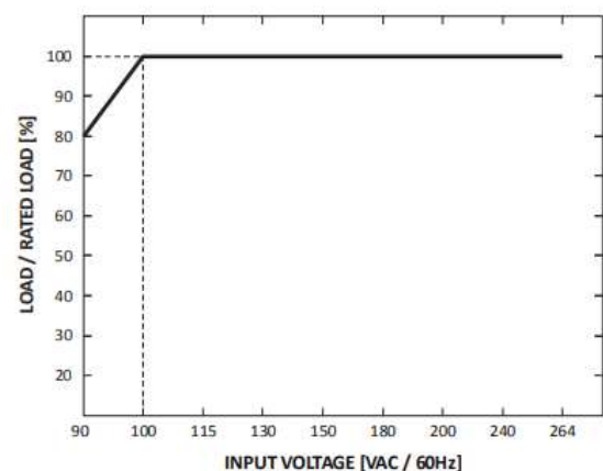
STATIC CHARACTERISTICS
