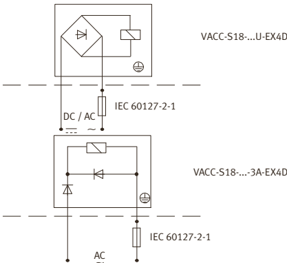
Fig. 2 Electrical connection diagram
