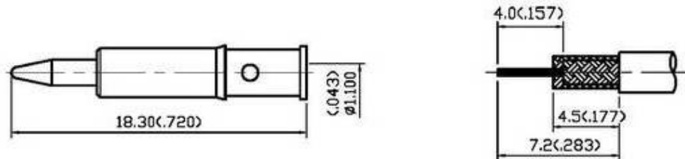
STRIPPING DIMENSION
