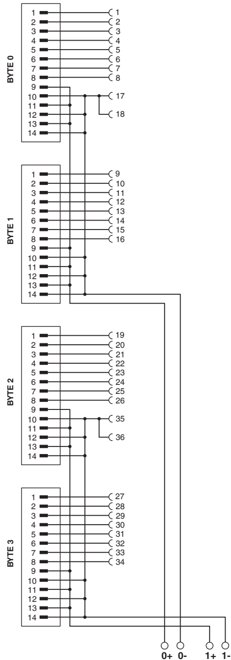
Circuit diagram
