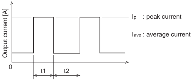
Fig.5.1 Peak current
