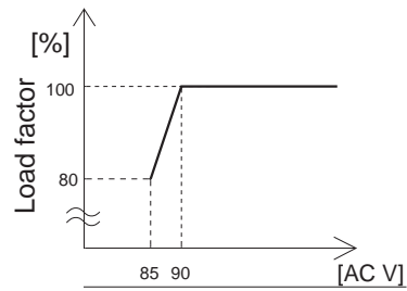
Fig.3.14 Derating curve depending on input voltage
