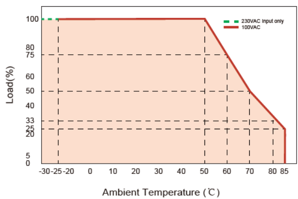
Derating Curve
