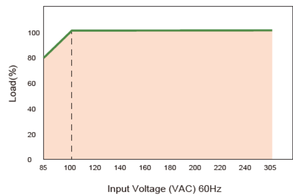
Static Characteristics
