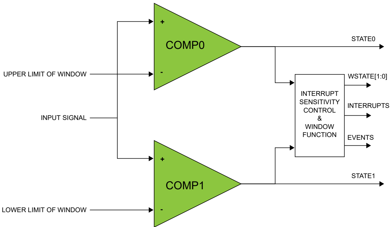
Figure 37-4. Comparators in Window Mode
