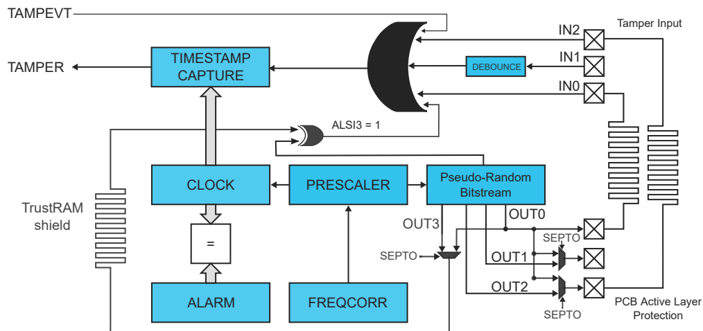
Figure 23-4. RTC Block Diagram (Tamper Detection Use Case)
