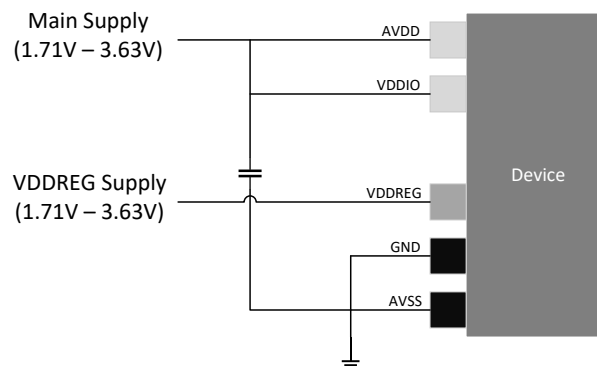
Figure 7-3. Power Supply for Dual Voltage Mode
