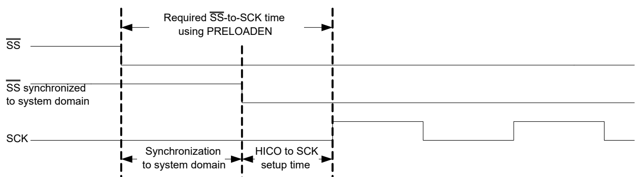
Figure 32-31. Timing Using Preloading
