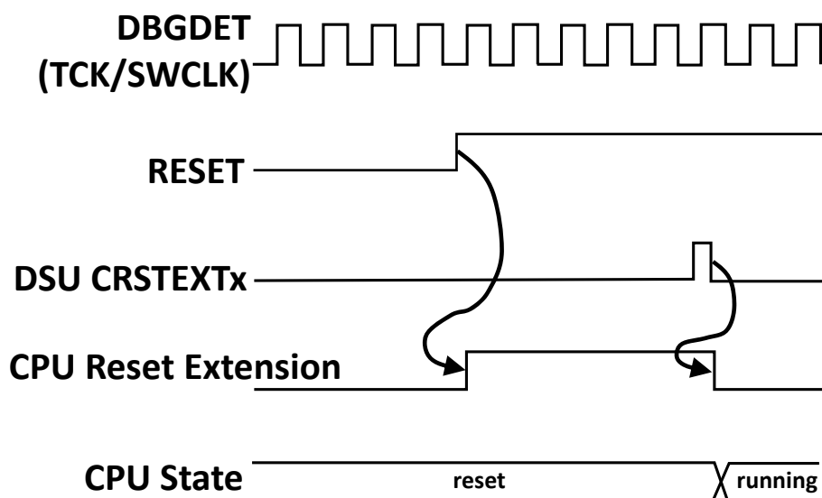
Figure 15-4. Typical CPU Reset Extension Set and Clear Timing Diagram
