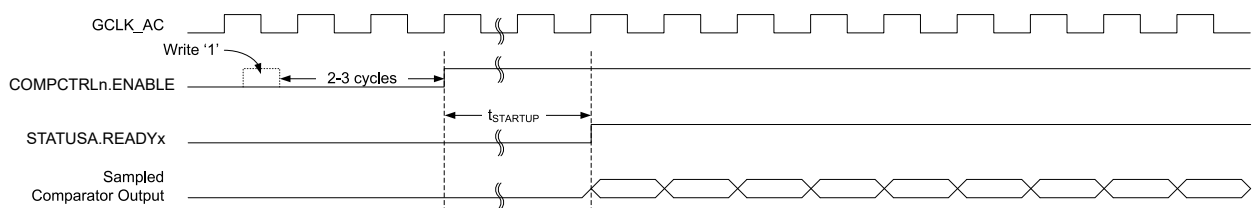
Figure 37-2. Continuous Measurement Example
