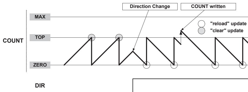
Figure 38-2. Counter Operation
