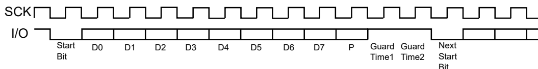
Figure 32-21. T=0 Protocol without Parity Error
