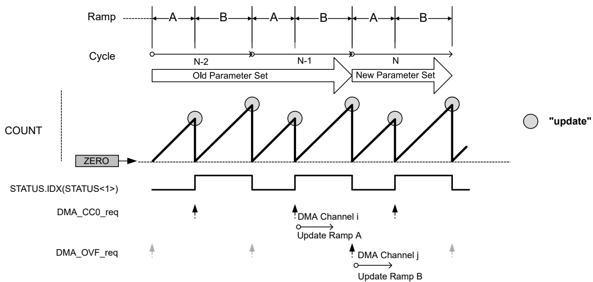
Figure 38-35. DMA Triggers in RAMP2 Operation and Circular Buffer Enabled
