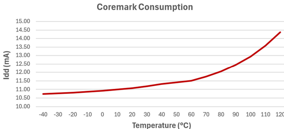
Figure 41-1. Power Consumption over Temperature in Active Mode (Typical values for guidance only, not tested)
