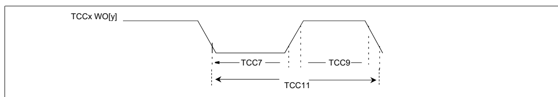
Figure 41-12. TCCx Timer Compare Output Module AC Timing Diagrams
