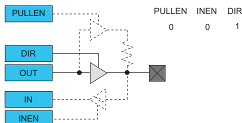
Figure 31-6. I/O Configuration - Totem-Pole Output with Disabled Input
