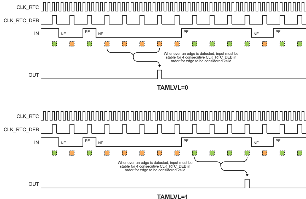
Figure 23-7. Edge Detection with Synchronous Stability Debouncing
