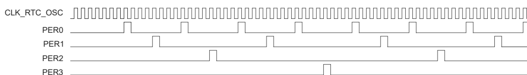
Figure 23-5. Example Periodic Events
