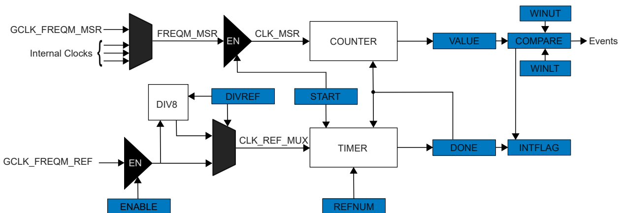
Figure 22-1. FREQM Block Diagram
