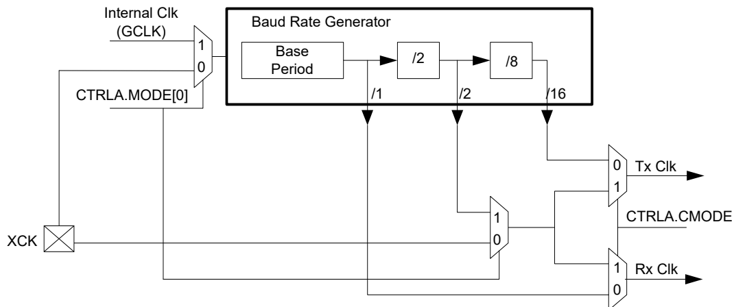
Figure 32-9. Clock Generation
