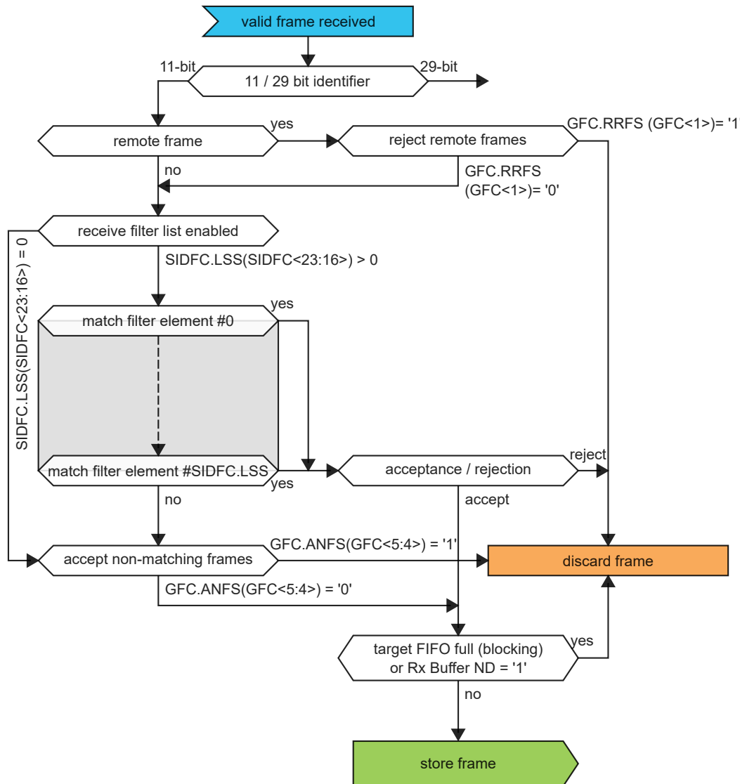
Figure 33-5. Standard Message ID Filtering
