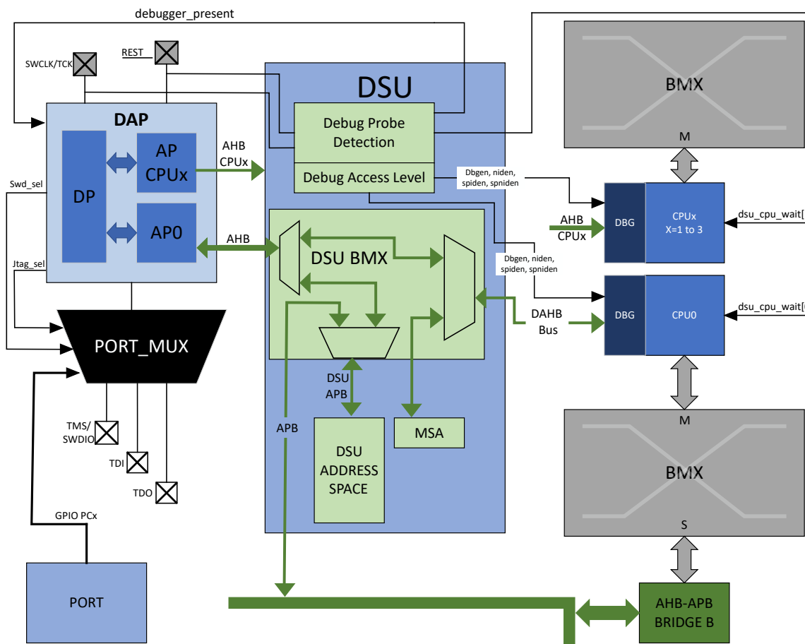
Figure 15-1. Block Diagram
