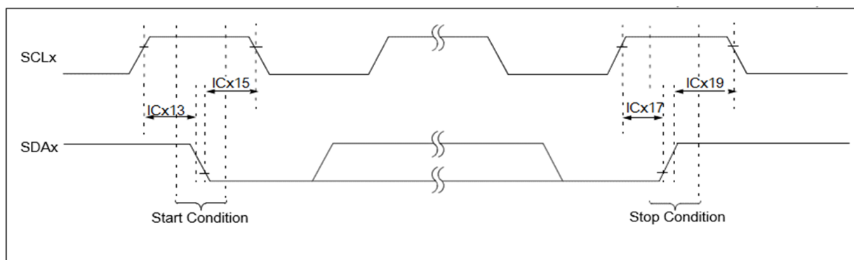
Figure 40-23. I 2 C Start/Stop Bits Client Mode AC Timing Diagrams
