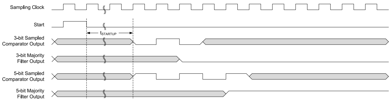
Figure 37-7. Single-Shot Filtering
