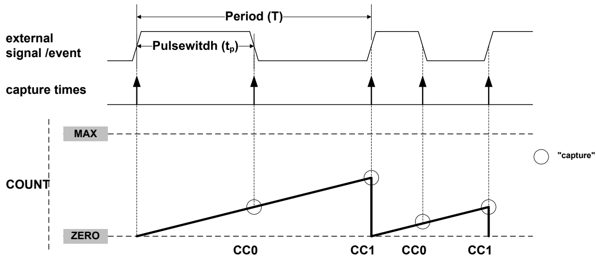
Figure 38-16. PWP Capture
