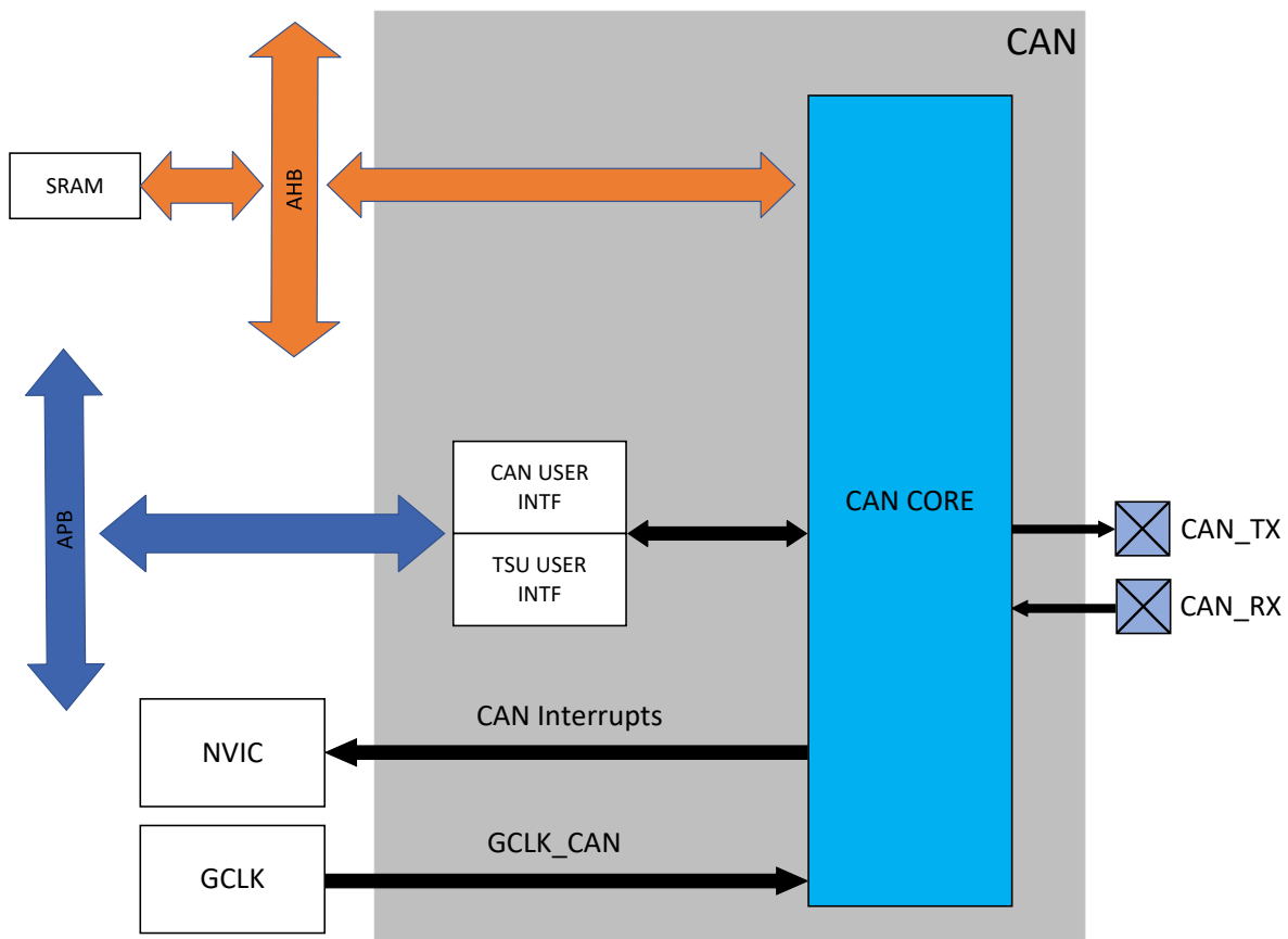
Figure 33-1. Block Diagram
