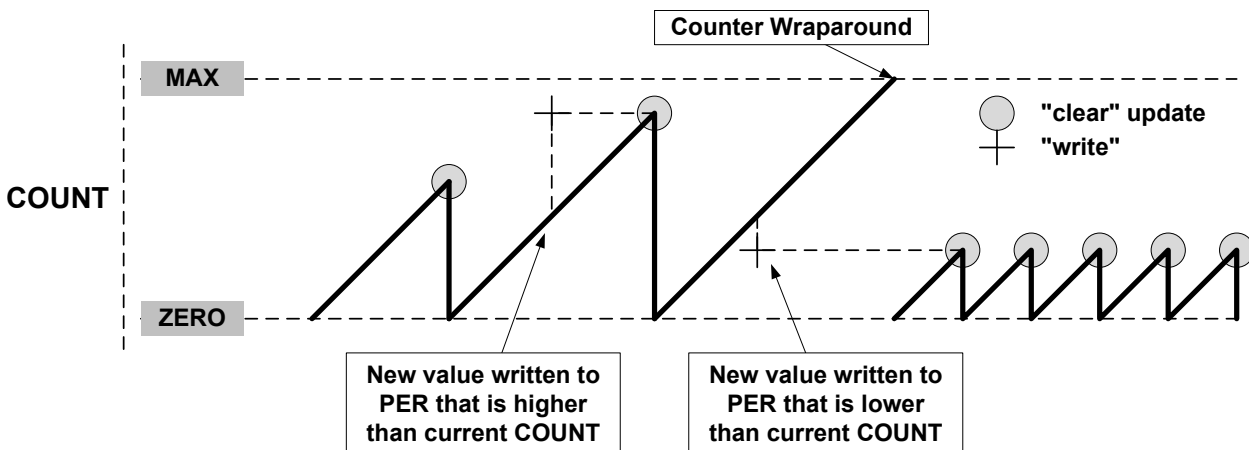
Figure 38-10. Unbuffered Single-Slope Up-Counting Operation
