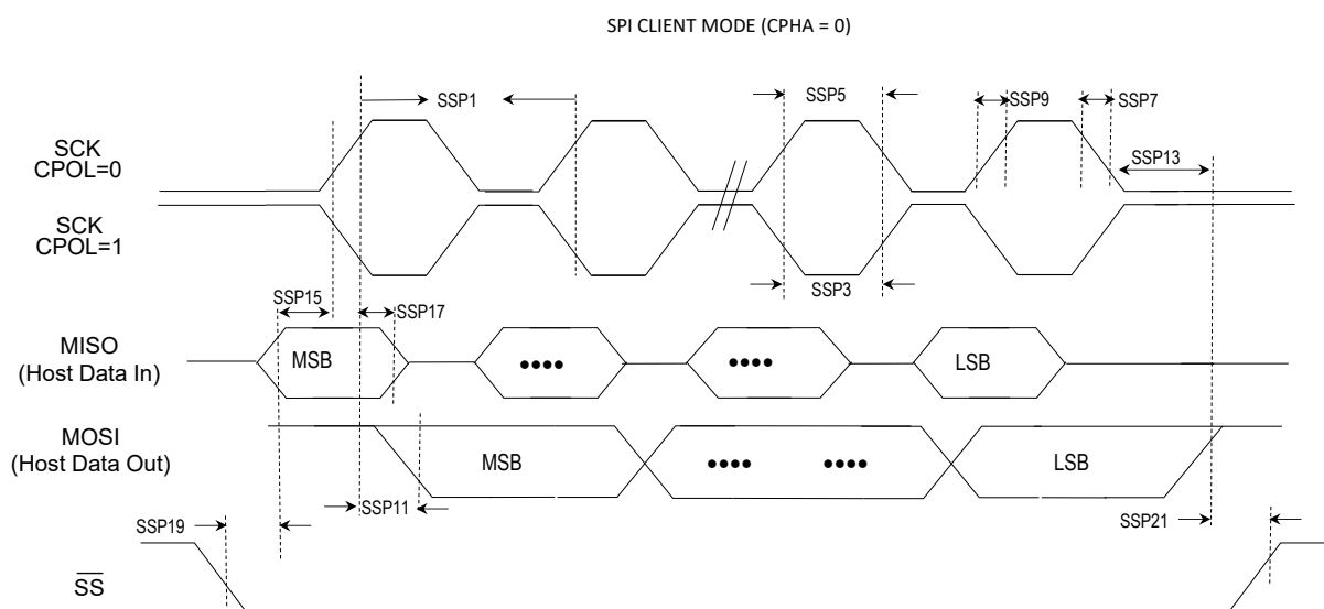
Figure 40-19. SPIx Client Module (CPHA = 0) Timing Diagrams
