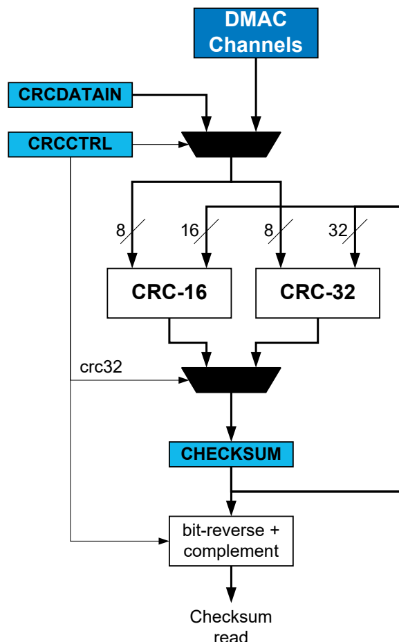
Figure 24-15. CRC Generator Block Diagram
