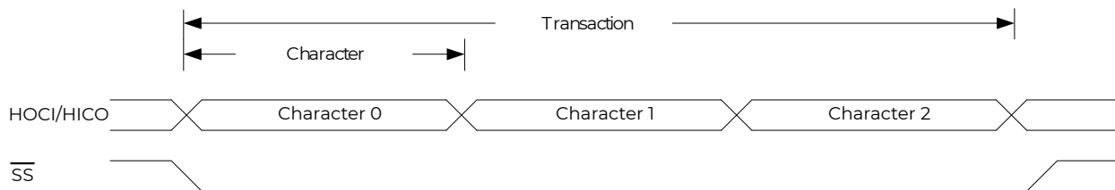
Figure 32-29. SPI Transaction Format
