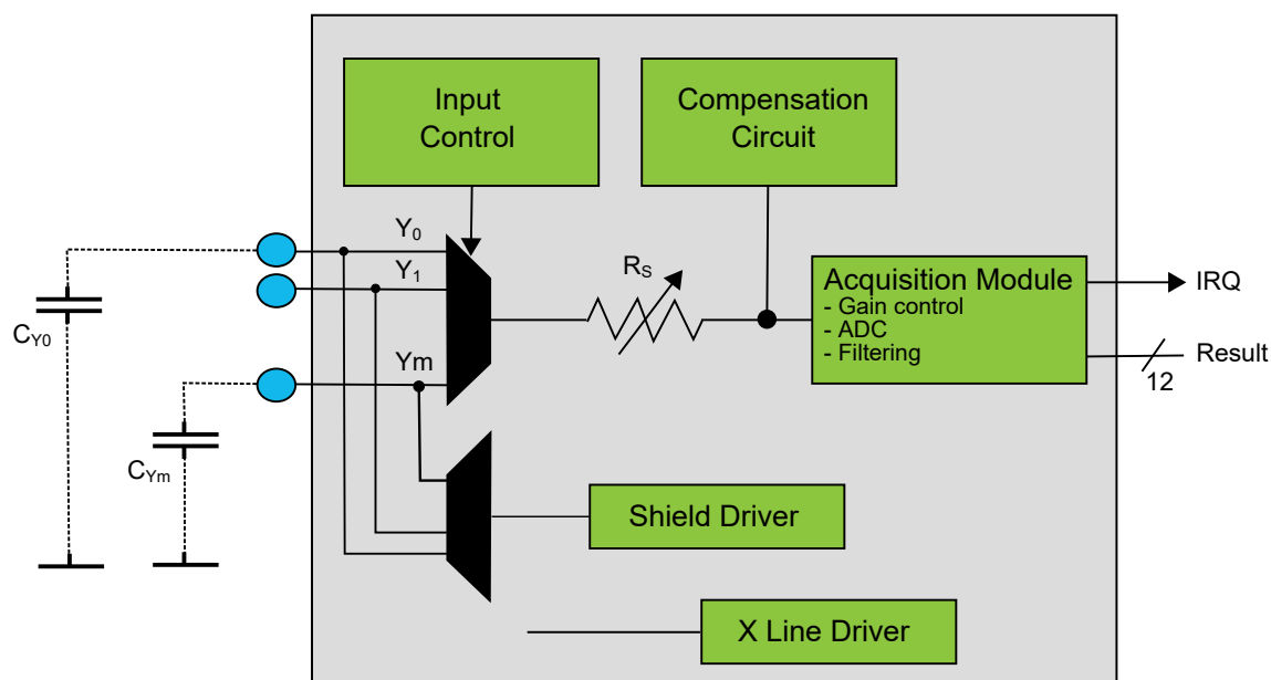
Figure 39-2. PTC Block Diagram Self Capacitance
