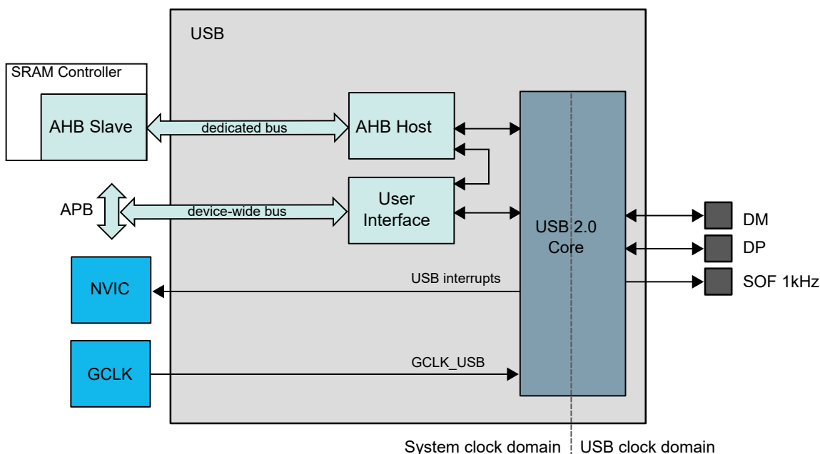
Figure 34-1. LS/FS Implementation: USB Block Diagram
