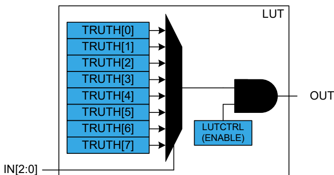
Figure 35-2. Truth Table Output Value Selection
