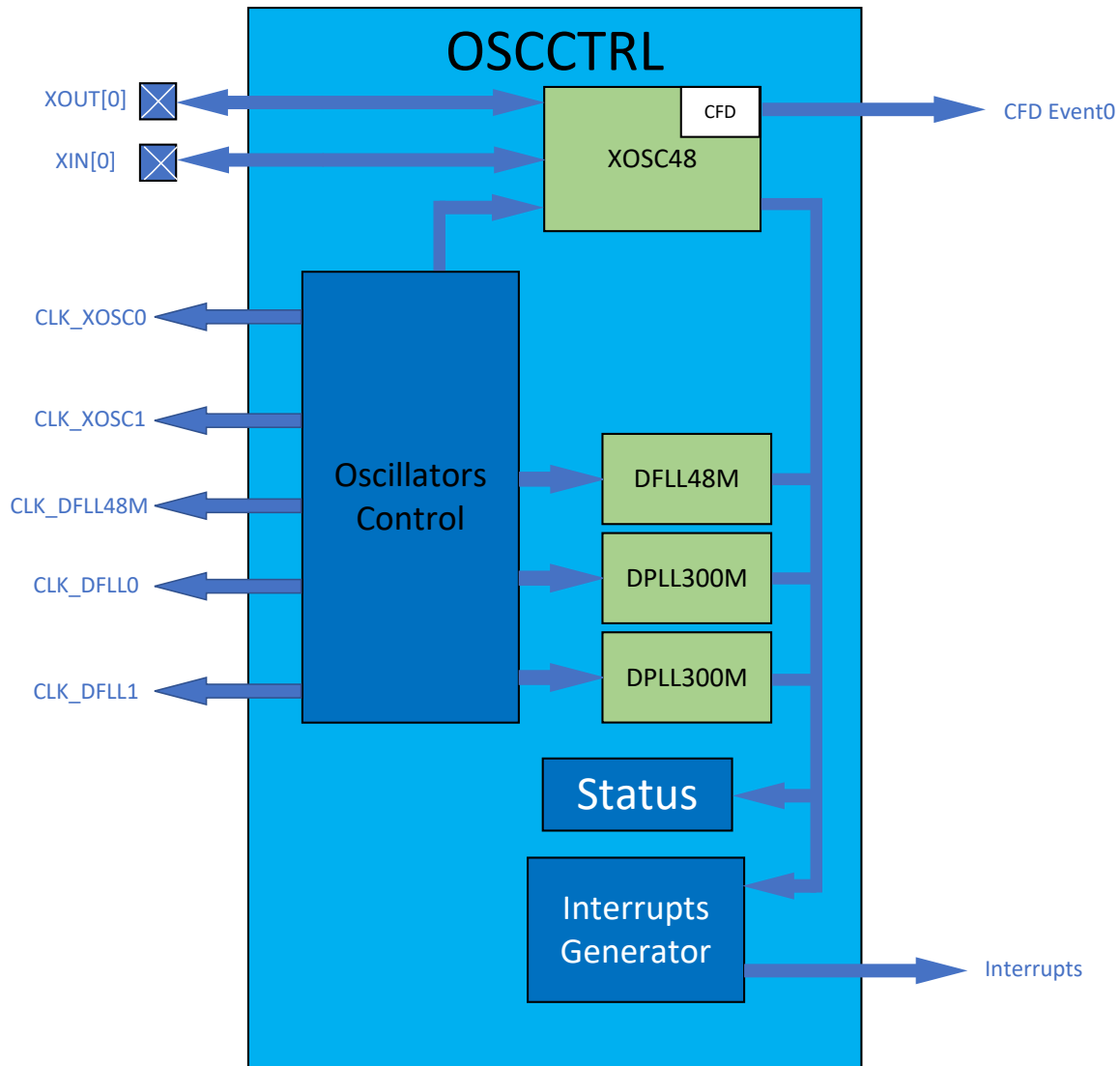
Figure 17-1. OSCCTRL Block Diagram
