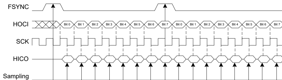
Figure 32-42. FMODE = CLIENT, FSPOL = HIGH, FSLEN = STROBE, FSES = 0
