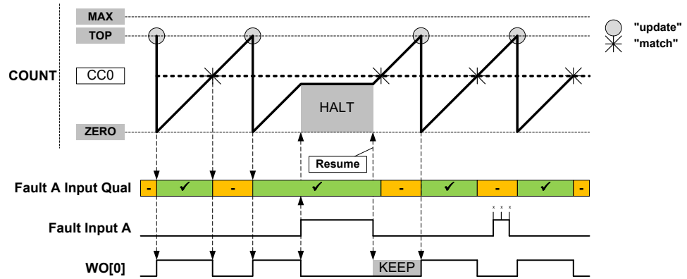
Figure 38-32. Waveform Generation with Fault Qualification, Halt, and Restart Actions
