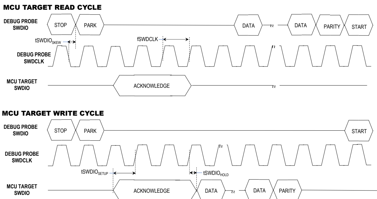
Figure 40-30. SWD 2-Wire Read/Write AC Timing Diagrams
