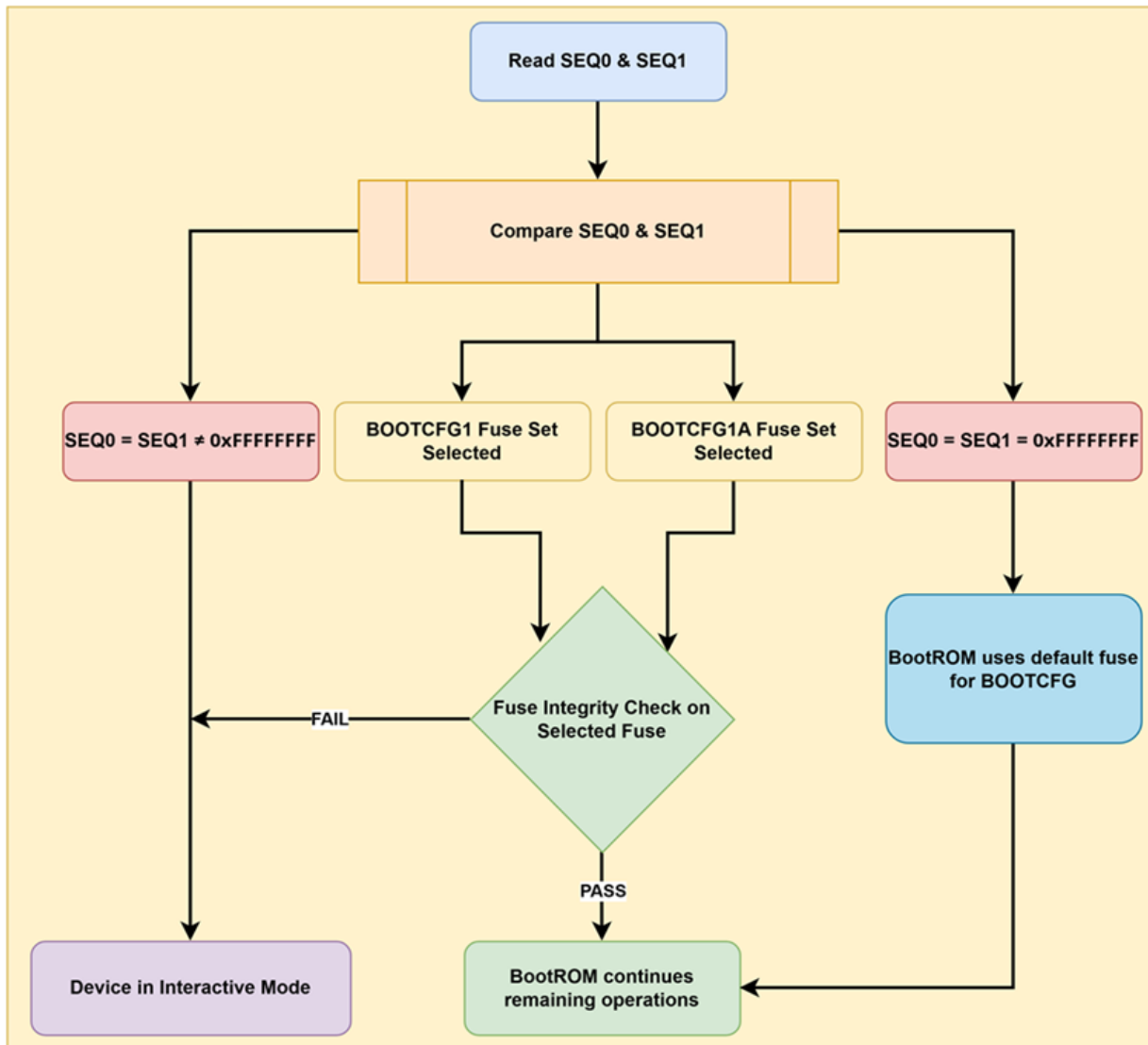
Figure 12-6. USERCFG1/1x fuse Integrity Check Selection
