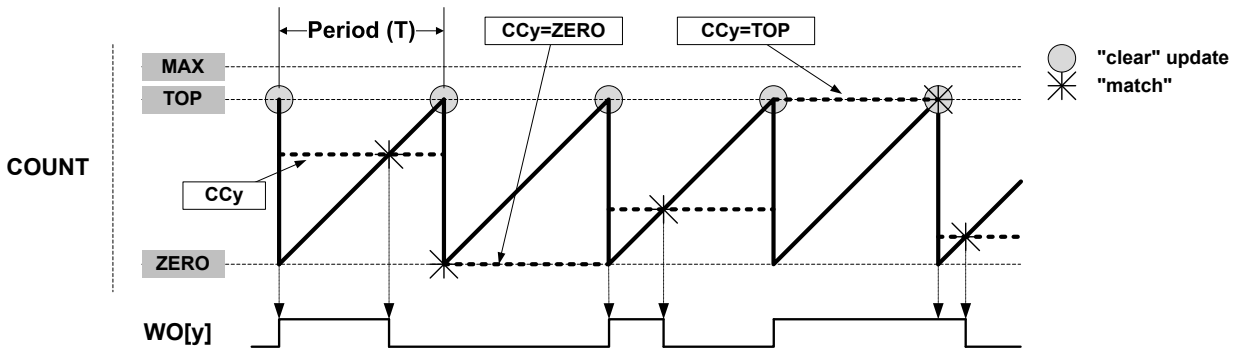
Figure 38-5. Single-Slope PWM Operation
