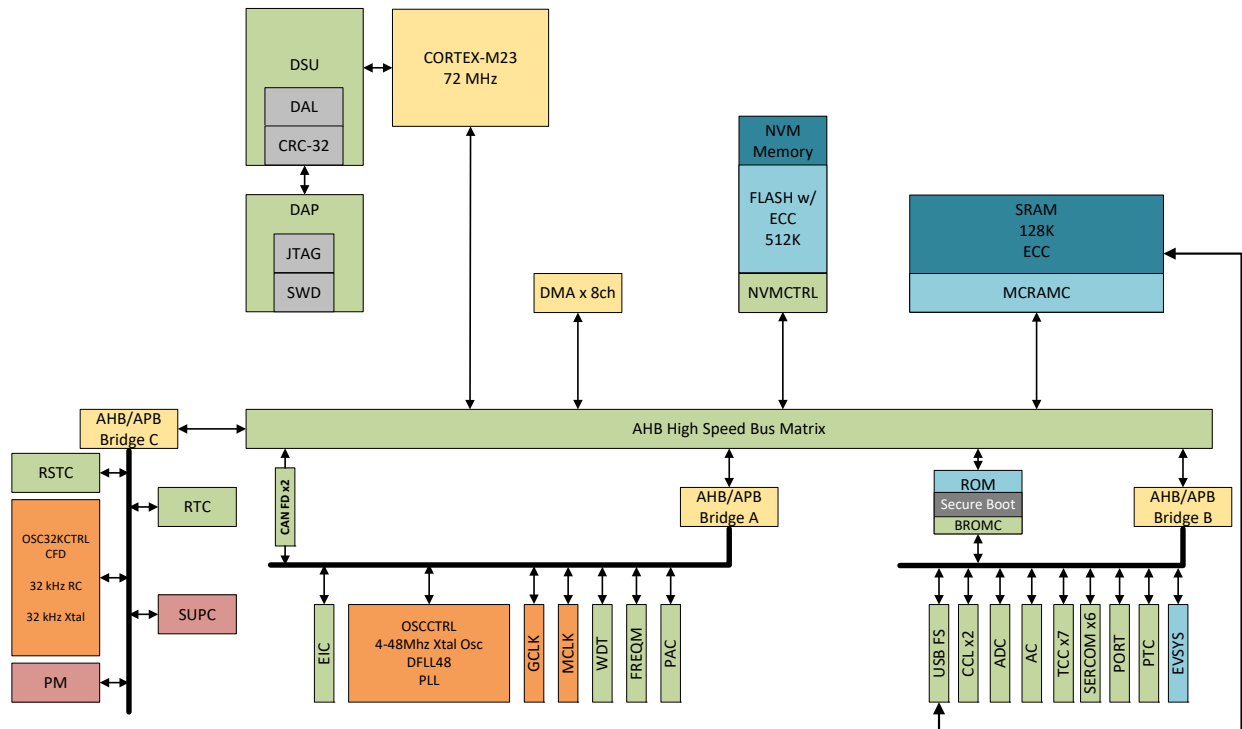
Figure 4-1. PIC32CM GC00 Block Diagram
