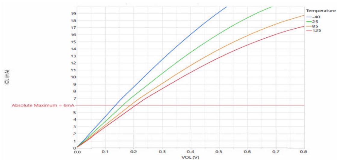
Figure 40-10. IOL vs VOL, 8x Drive Strength I/O on Typical parts with VDDIO = 3.0 V
