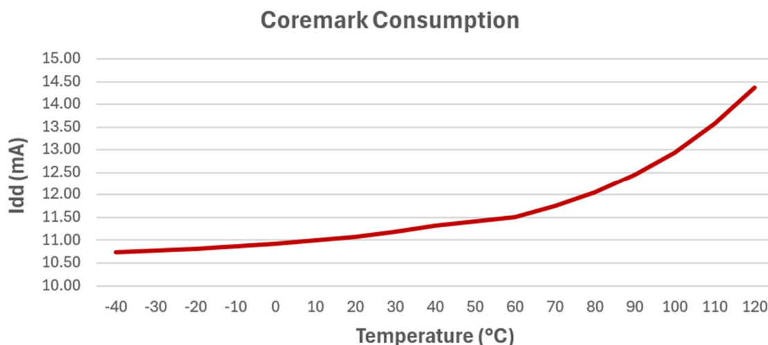
Figure 40-1. Power Consumption over Temperature in Active Mode (Typical values for guidance only, not tested)
