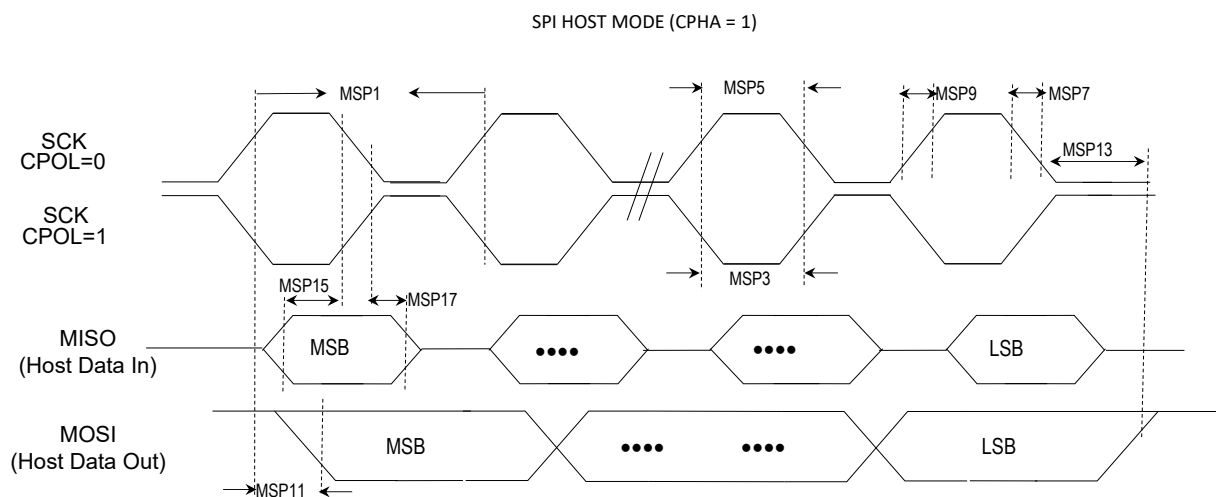
Figure 40-18. SPIx Host Module (CPHA = 1) Timing Diagrams
