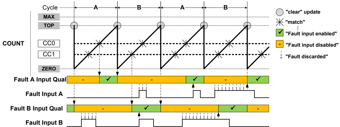
Figure 38-25. Fault Qualification in RAMP2 Operation with Inverted Polarity
