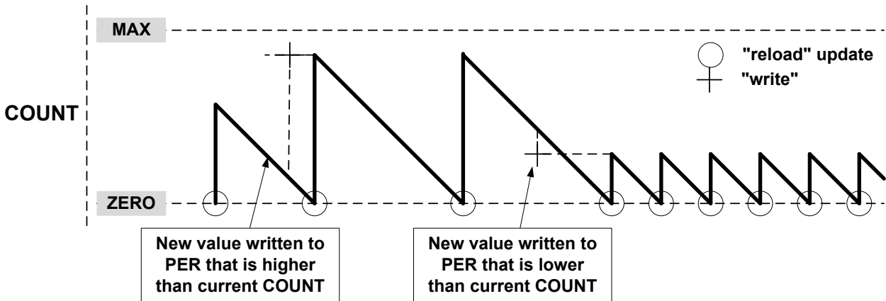
Figure 38-11. Unbuffered Single-Slope Down-Counting Operation
