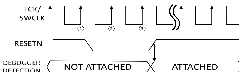
Figure 15-2. Cold-Plugging Timing Diagram
