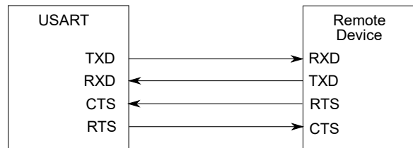
Figure 32-13. Connection with a Remote Device for Hardware Handshaking
