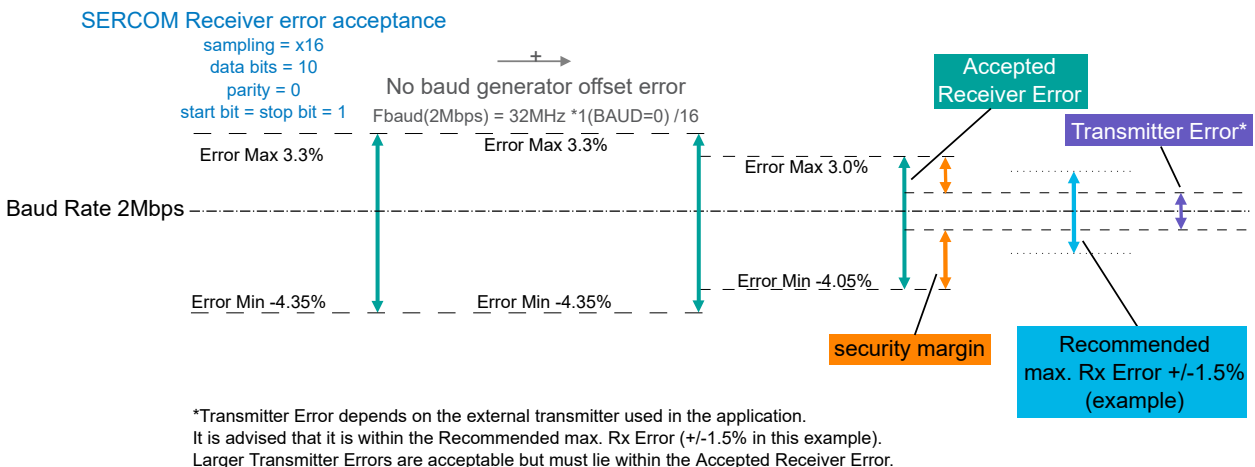
Figure 32-12. USART Rx Error Calculation Example
