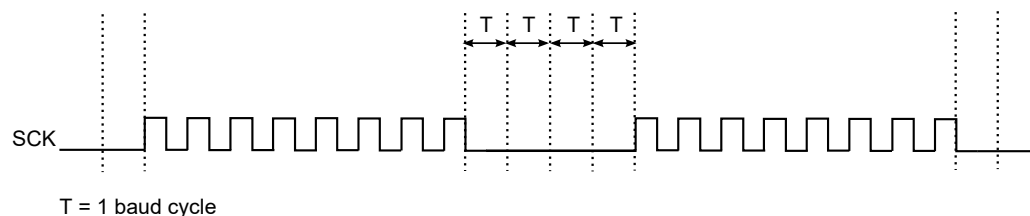
Figure 32-35. Four Cycle Inter-Character Spacing Example
