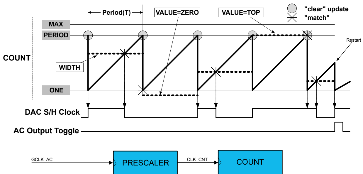
Figure 37-5. Sample and Hold Clock Generation
