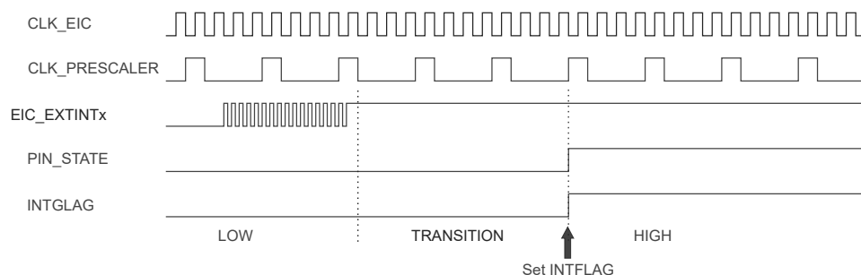
Figure 28-3. EIC_EXTINTx Pin Synchronous Debouncing (Rising Edge)
