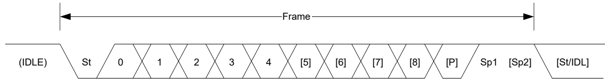
Figure 32-8. Frame Formats
