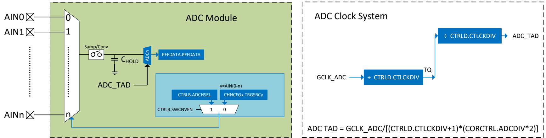
Figure 36-1. ADC Block Diagram
