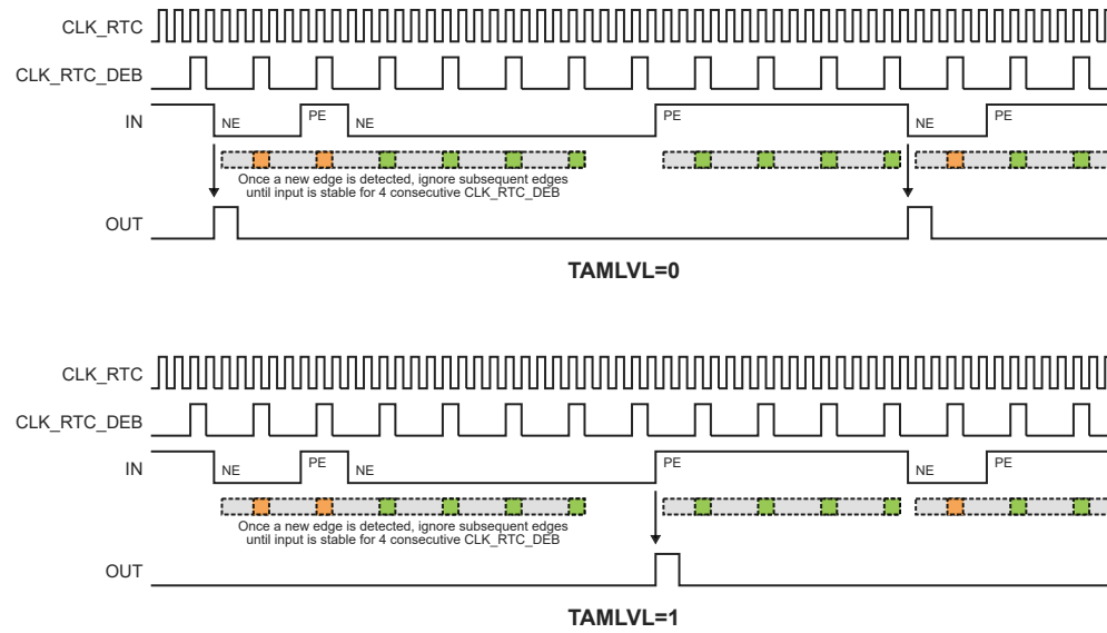
Figure 23-8. Edge Detection with Asynchronous Stability Debouncing
