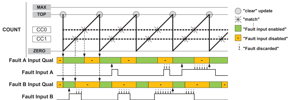
Figure 38-24. Fault Qualification in RAMP1 Operation
