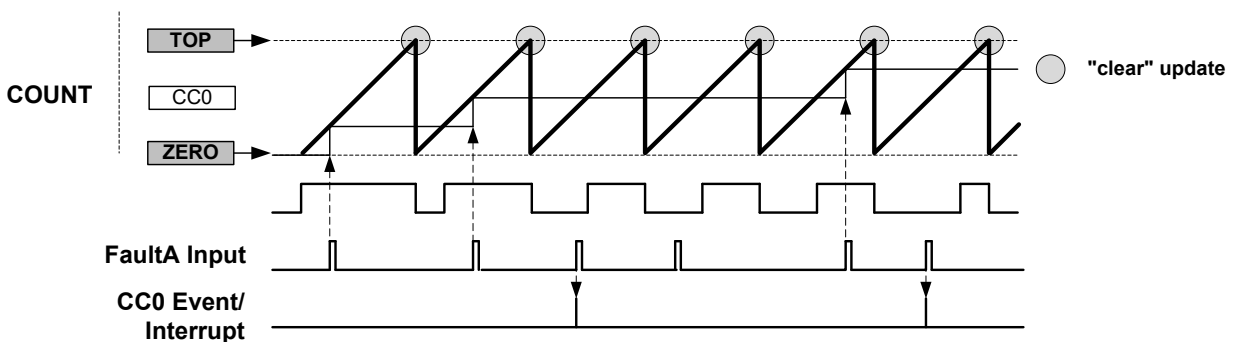
Figure 38-29. Capture Action "CAPTMAX"
