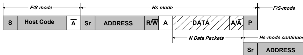
Figure 32-51. High Speed Transfer
