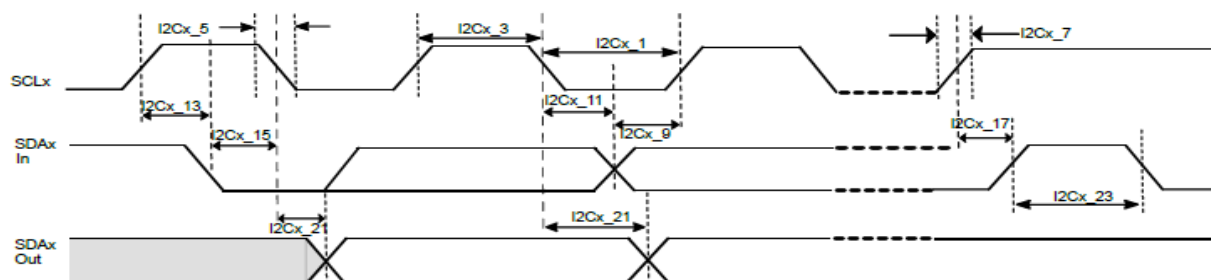
Figure 40-24. I 2 C Bus Data Client Mode AC Timing Diagrams
