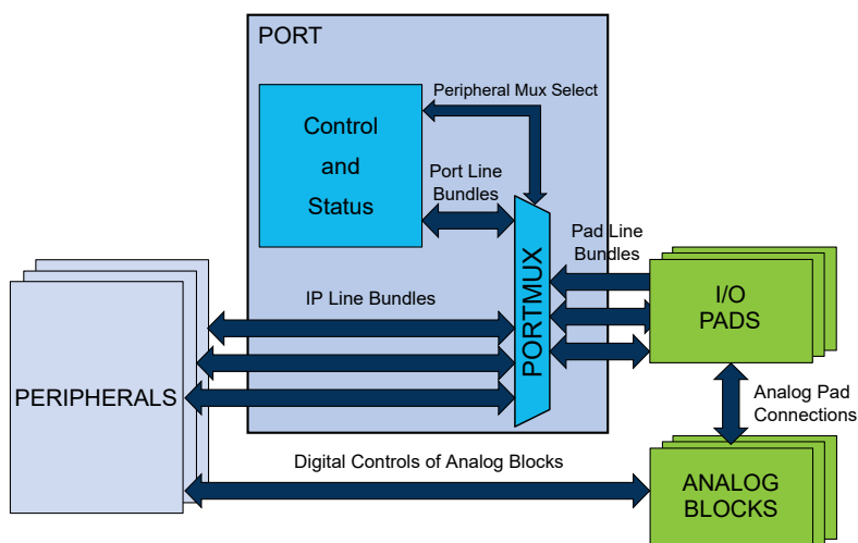
Figure 31-1. PORT I/O Block Diagram
