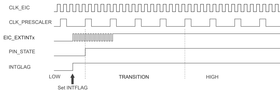
Figure 28-4. EIC_EXTINTx Pin(s) Asynchronous Debouncing (Rising Edge)
