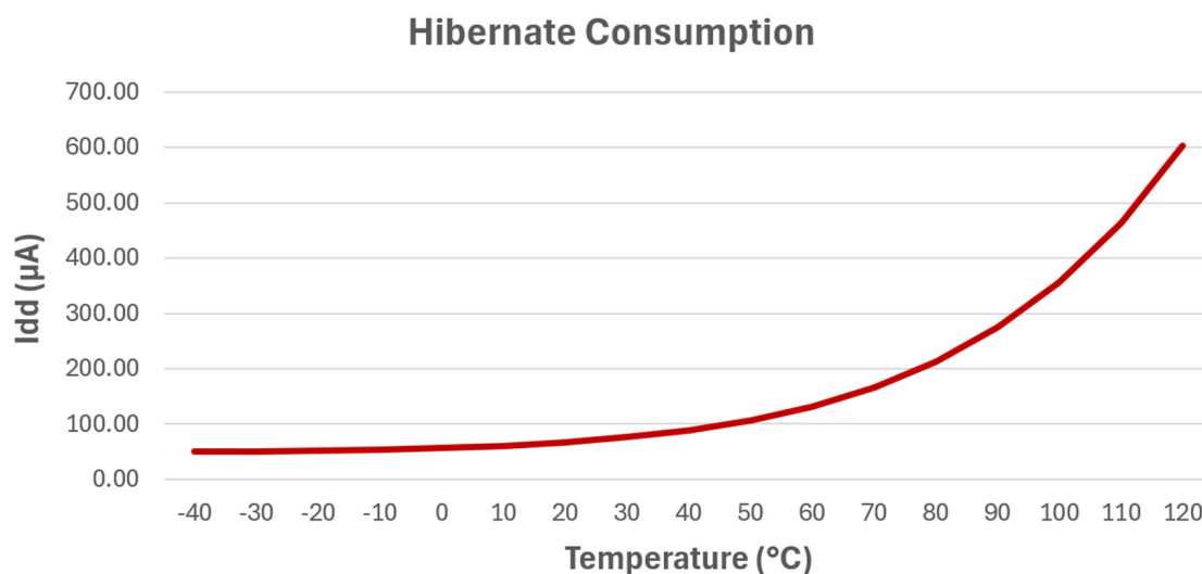
Figure 40-4. Power Consumption over Temperature in Hibernate Mode (Typical values for guidance only, not tested)
