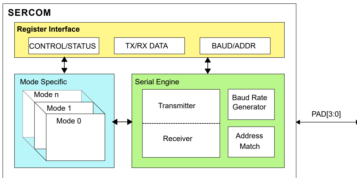
Figure 32-1. SERCOM Block Diagram
