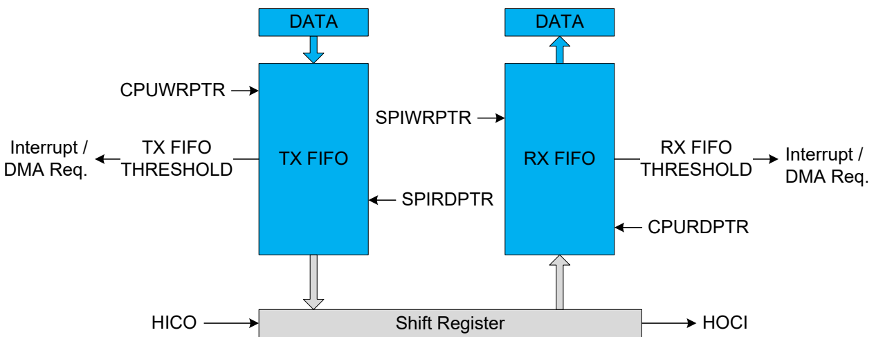
Figure 32-43. FIFO Overview
