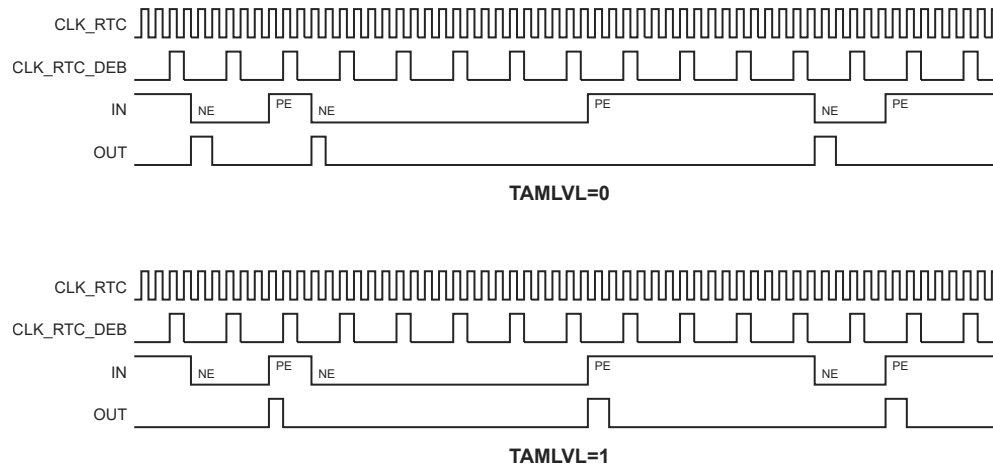
Figure 23-6. Edge Detection with Debouncer Disabled
