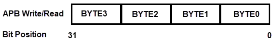
Figure 32-25. 32-bit Extension Ordering
