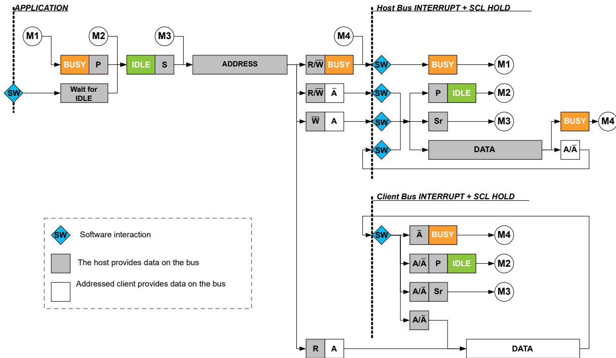
Figure 32-48. I 2 C Host Behavioral Diagram (SCLSM=0)
