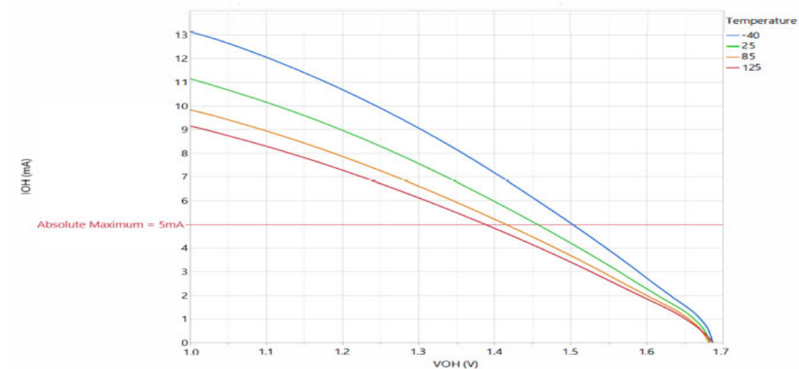
Figure 40-11. IOH vs VOH, 4x Drive Strength I/O on Typical parts with VDDIO = 1.71 V
