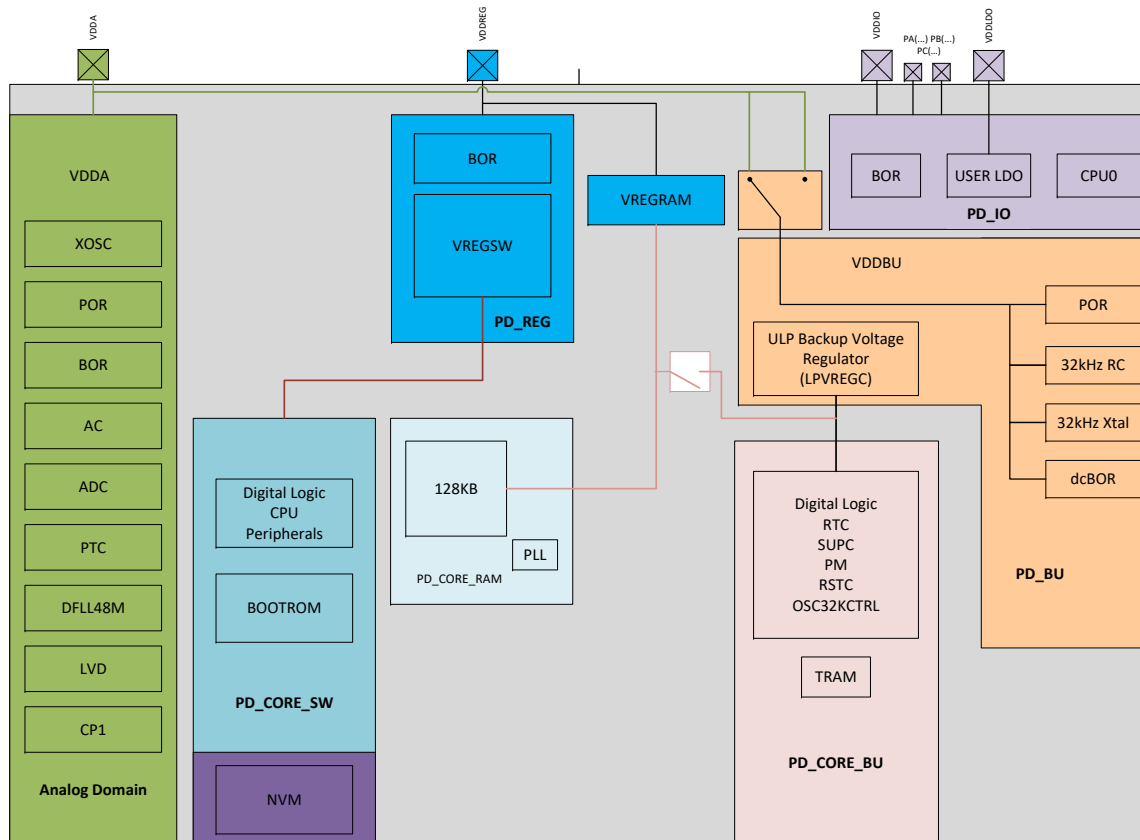
Figure 25-1. Supply Controller Block Diagram
