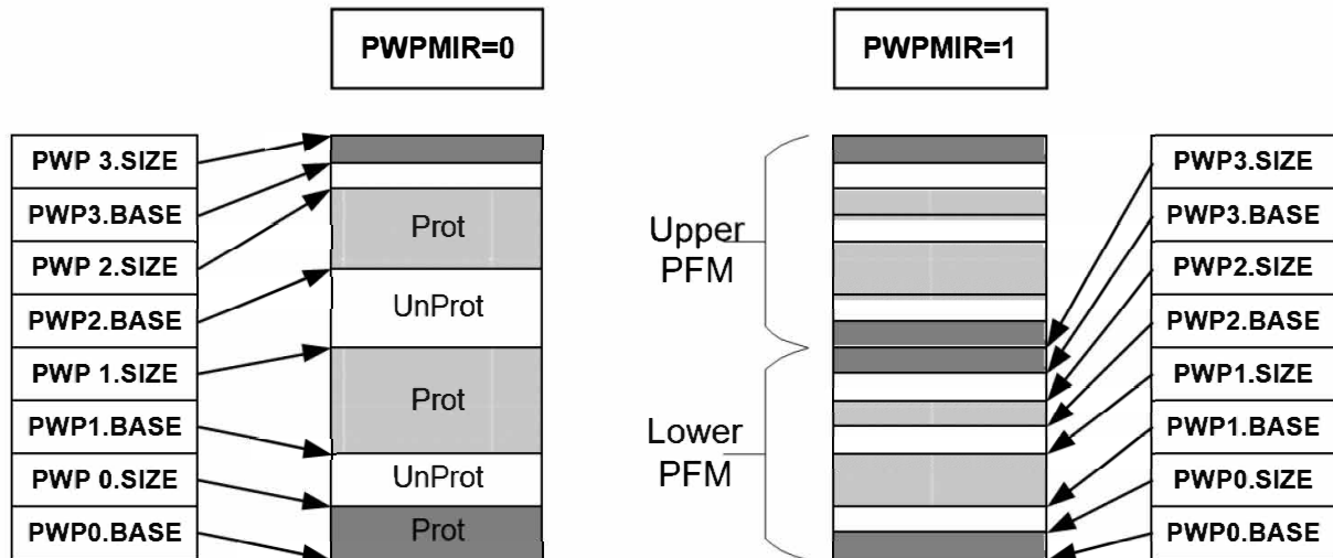
Figure 29-2. PWP Example: No Mirror versus Mirror
