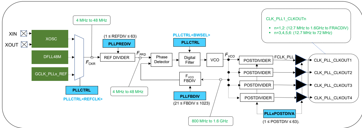
Figure 17-2. PLL Block Diagram
