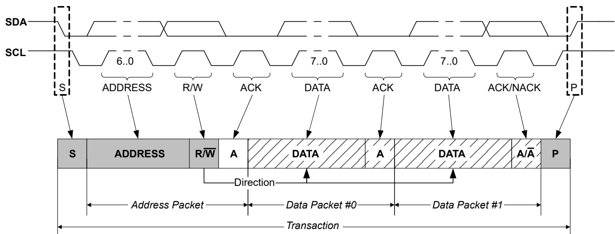
Figure 32-46. Basic I 2 C Transaction Diagram
