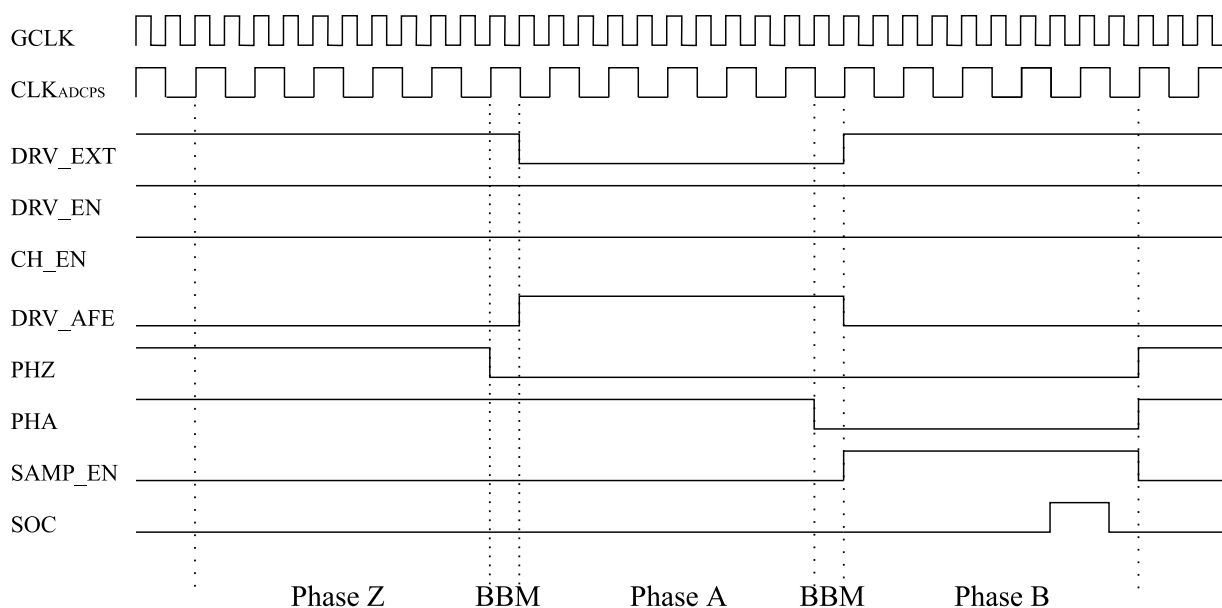
Figure 39-6. Differential Intergration of mutual cap sensor, normal polarity (CSD = 4)
