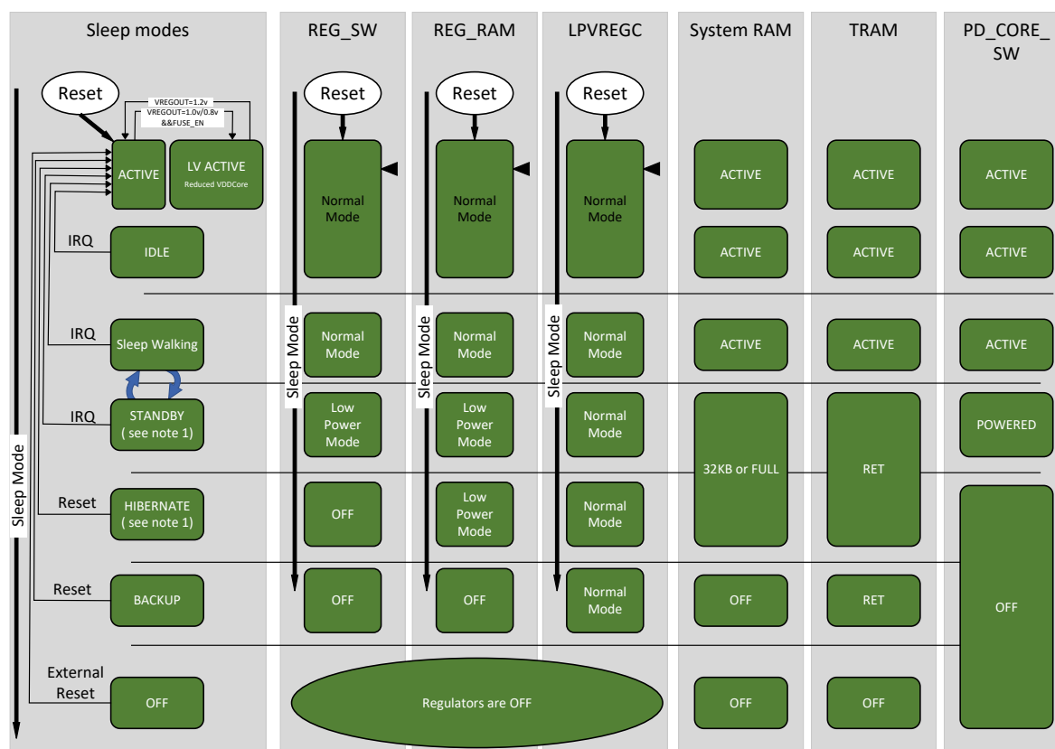
Figure 26-2. OPERATING CONDITIONS AND SLEEPWALKING
