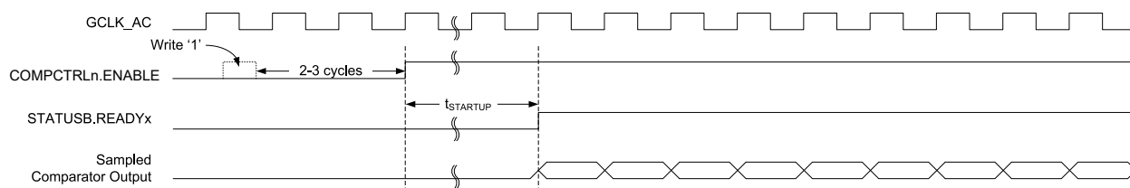
Figure 37-8. Continuous Mode SleepWalking
