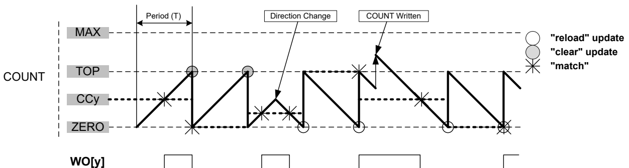
Figure 38-3. Normal Frequency Operation
