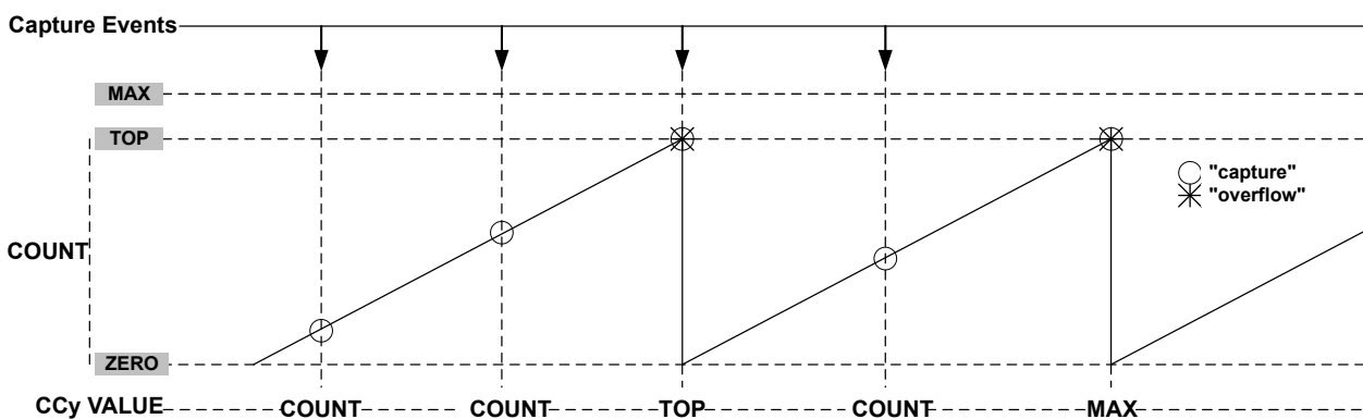
Figure 38-34. Time-Stamp
