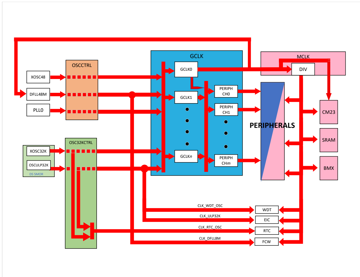
Figure 16-1. Clock Distribution Block Diagram
