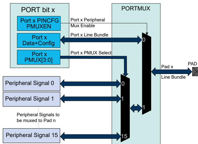
Figure 31-3. Overview of the Peripheral Functions Multiplexing
