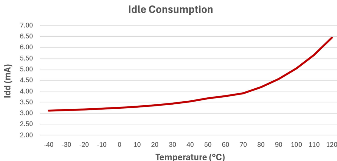
Figure 40-2. Power Consumption over Temperature in Idle mode (Typical values for guidance only, not characterized over process or voltage).
