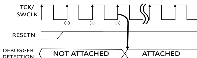
Figure 15-3. Hot-Plugging Detection Timing Diagram
