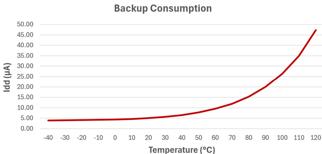
Figure 41-5. Power Consumption over Temperature in Backup Mode (Typical values for guidance only, not tested)
