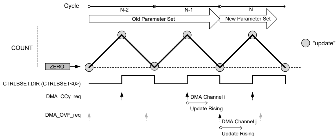
Figure 38-36. DMA Triggers in DSBOOTH Operation and Circular Buffer Enabled
