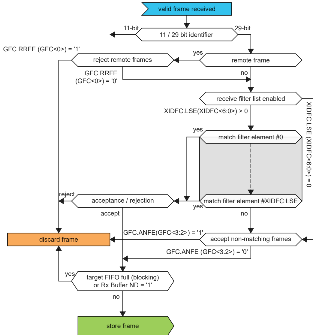
Figure 33-6. Extended Message ID Filtering
