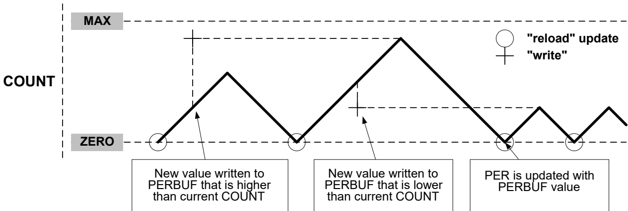
Figure 38-13. Changing the Period Using Buffering
