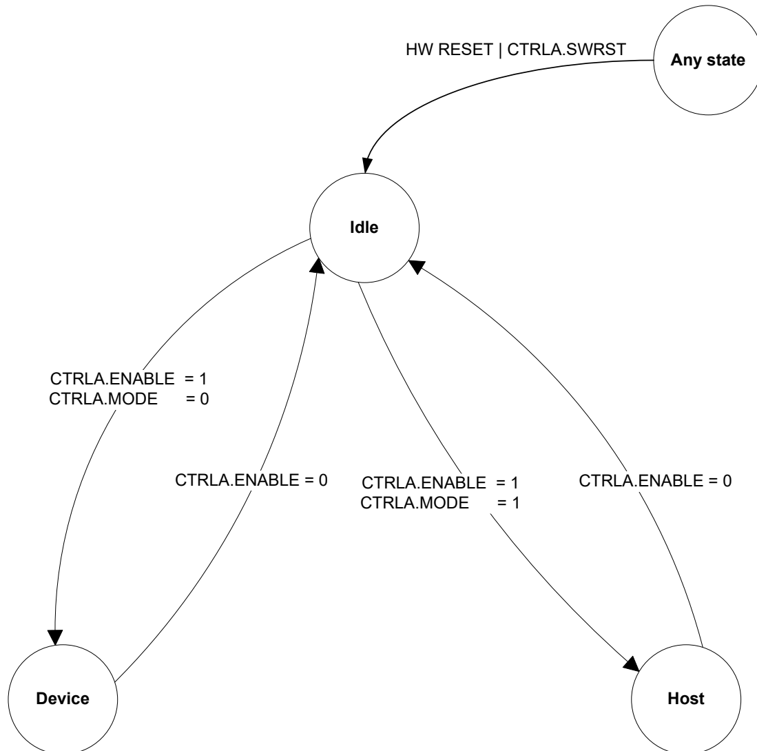
Figure 34-2. General States
