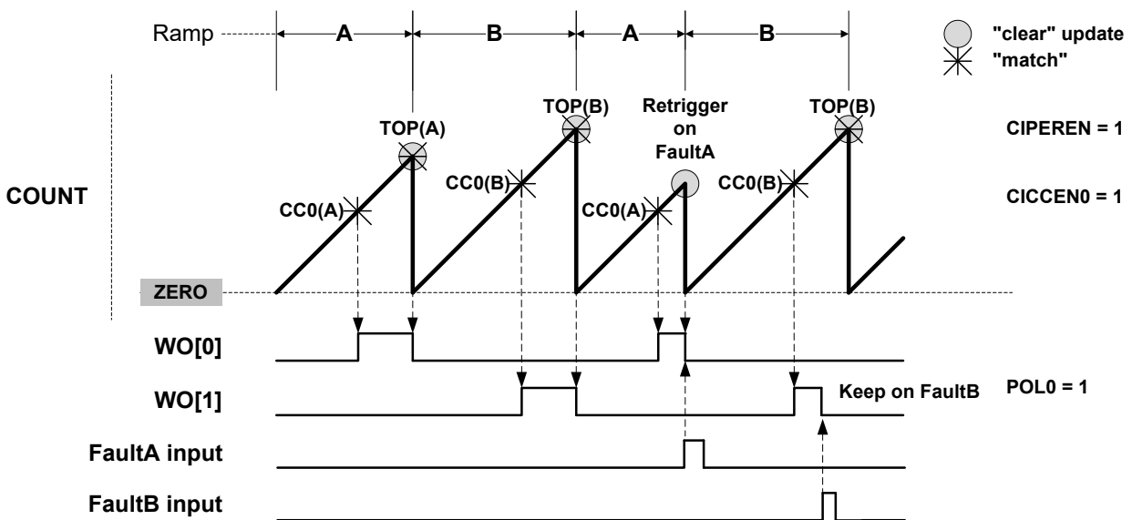
Figure 38-19. RAMP2 Alternate Operation
