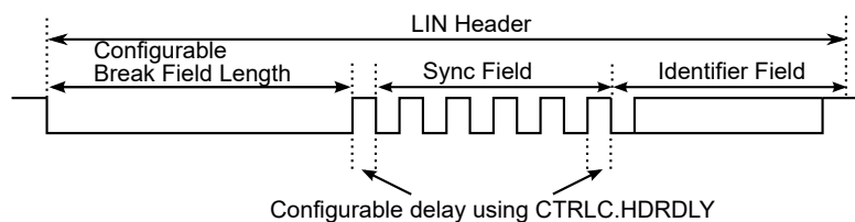
Figure 32-17. LIN Header Generation
