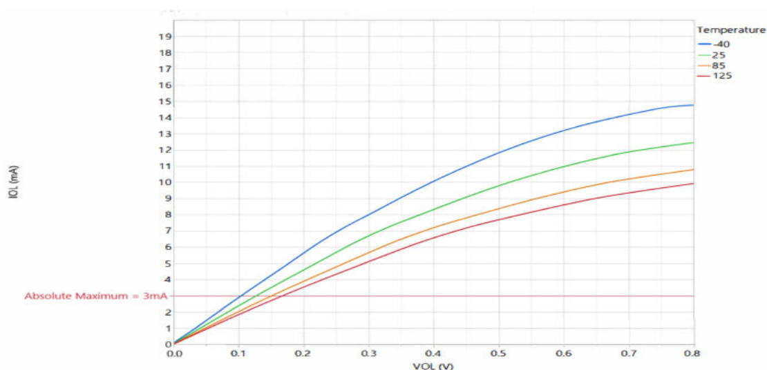
Figure 40-7. IOL vs VOL, 4x Drive Strength I/O on Typical parts with VDDIO = 1.71 V
