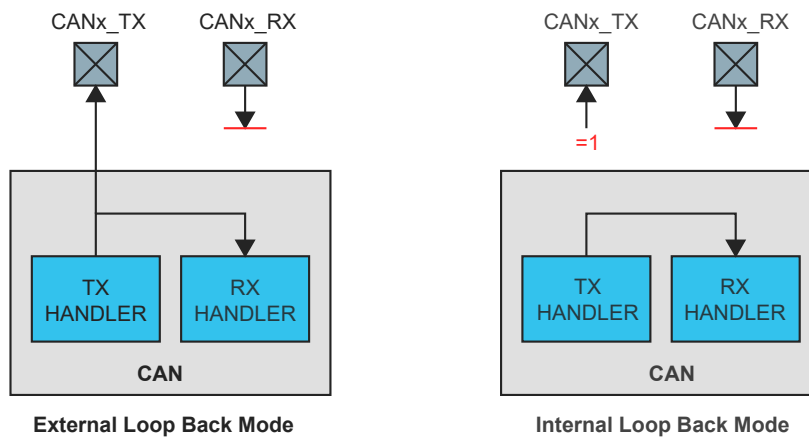
Figure 33-4. Pin Control in Loop Back Modes
