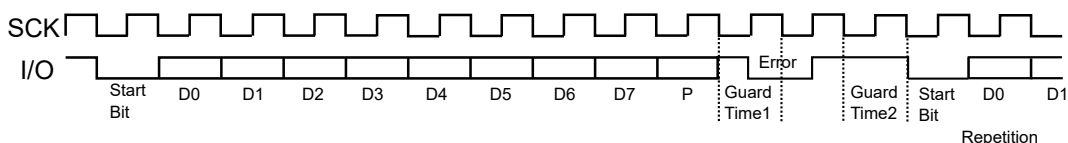
Figure 32-22. T=0 Protocol with Parity Error
