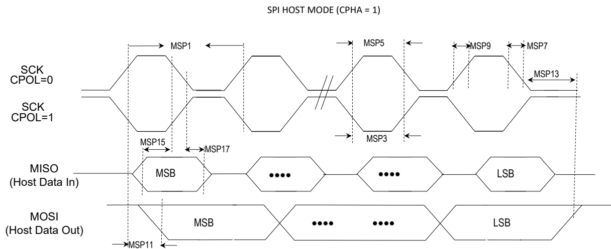
Figure 41-8. SPIx Host Module (CPHA = 1) Timing Diagrams
