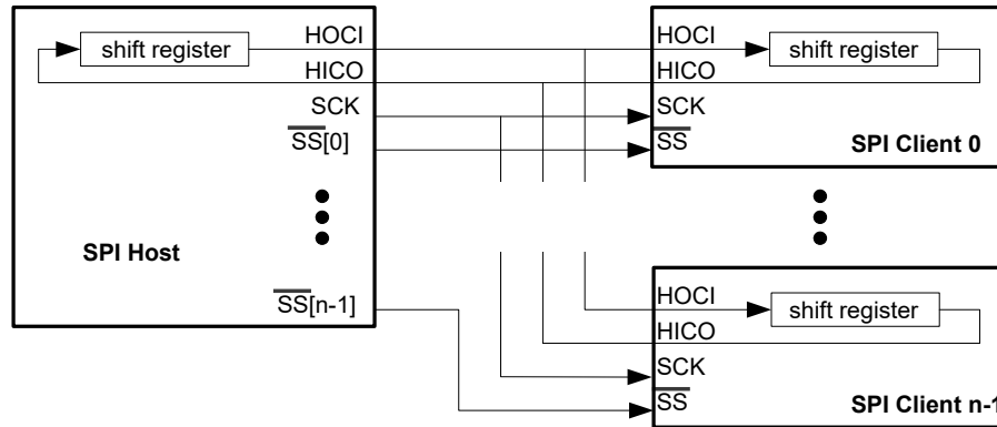
Figure 32-32. Multiple Clients in Parallel
