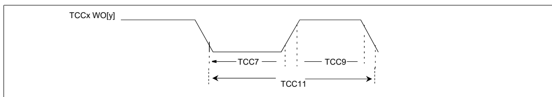
Figure 40-28. TCCx Timer Compare Fault Output Module AC Timing Diagrams
