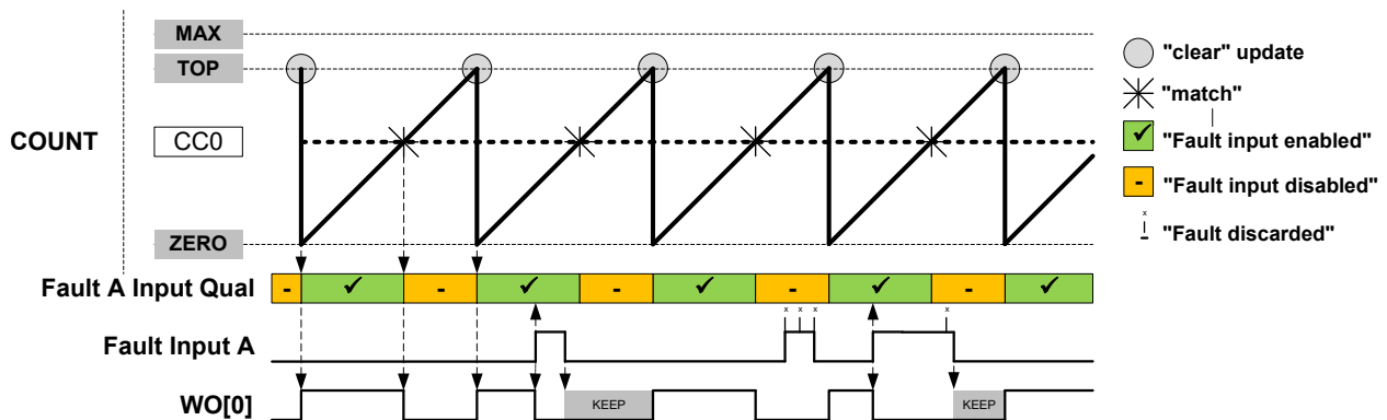
Figure 38-26. Waveform Generation with Fault Qualification and Keep Action
