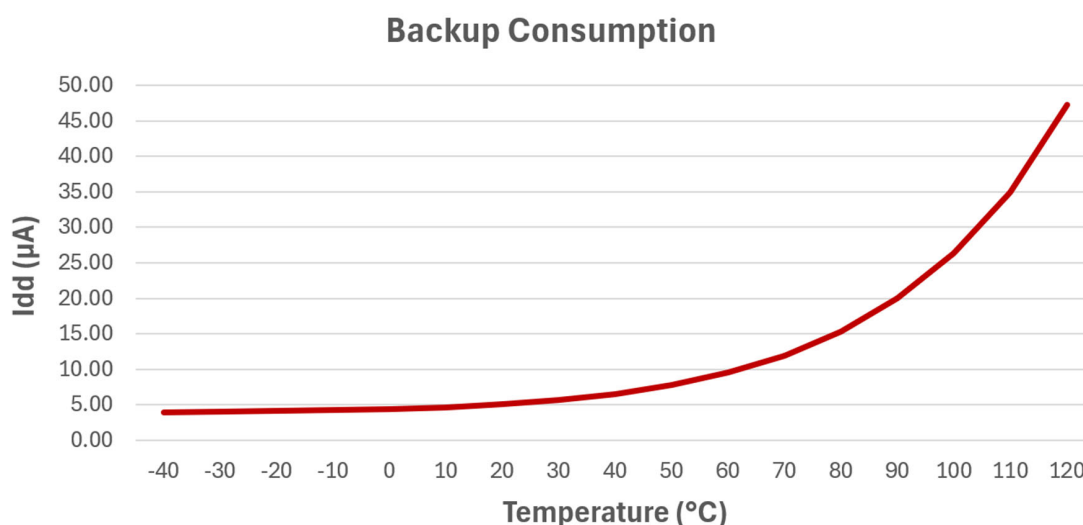
Figure 40-5. Power Consumption over Temperature in Backup Mode (Typical values for guidance only, not tested)
