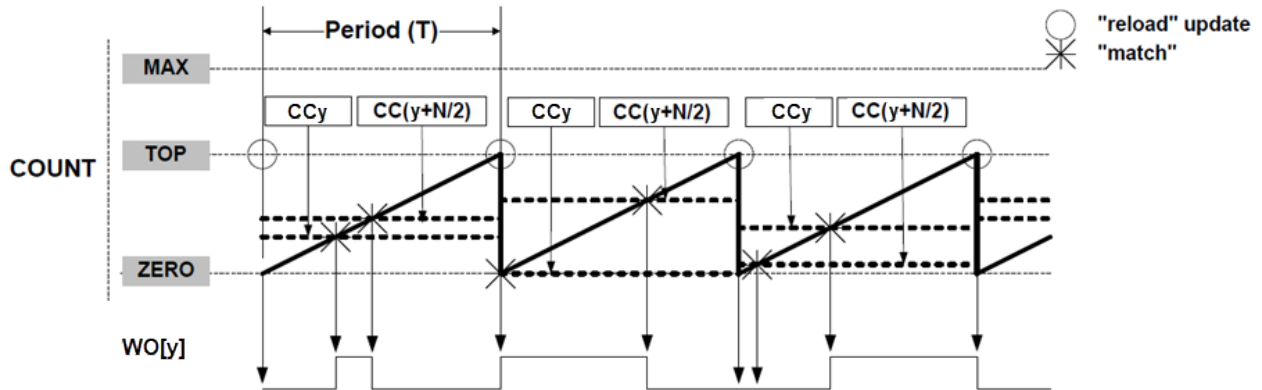
Figure 38-8. Dual-Compare Pulse Width Modulation ( N=CC\_NUM )
