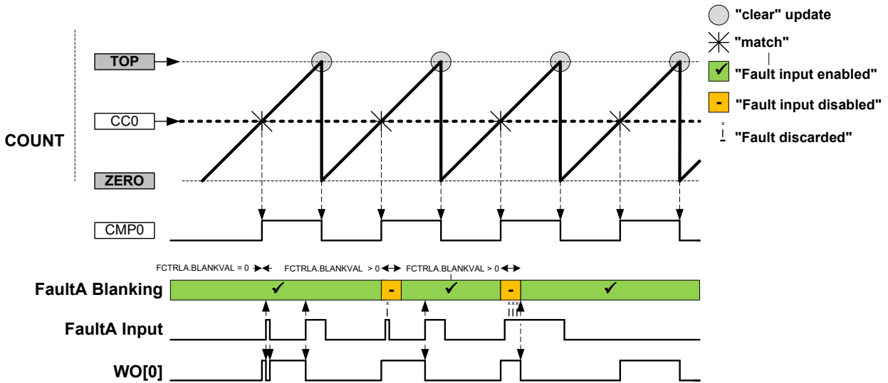
Figure 38-23. Fault Blanking in RAMP1 Operation with Inverted Polarity
