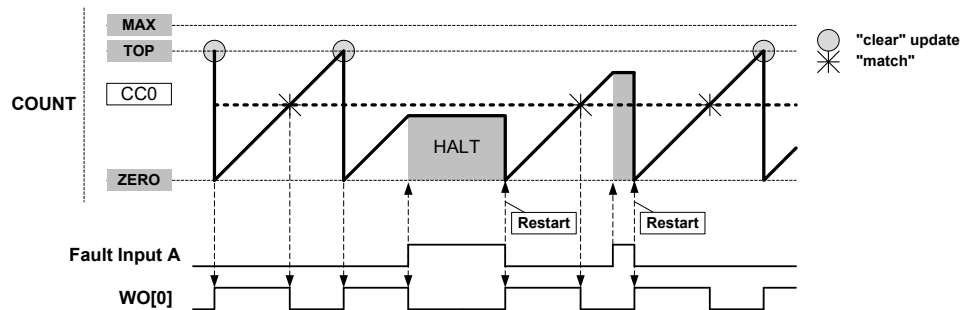
Figure 38-31. Waveform Generation with Halt and Restart Actions
