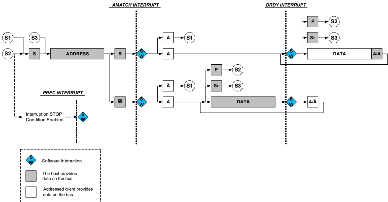
Figure 32-53. I 2 C Behavioral Diagram (SCLSM=0)
