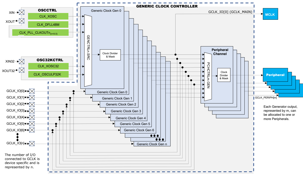
Figure 18-1. Device Clocking Diagram
