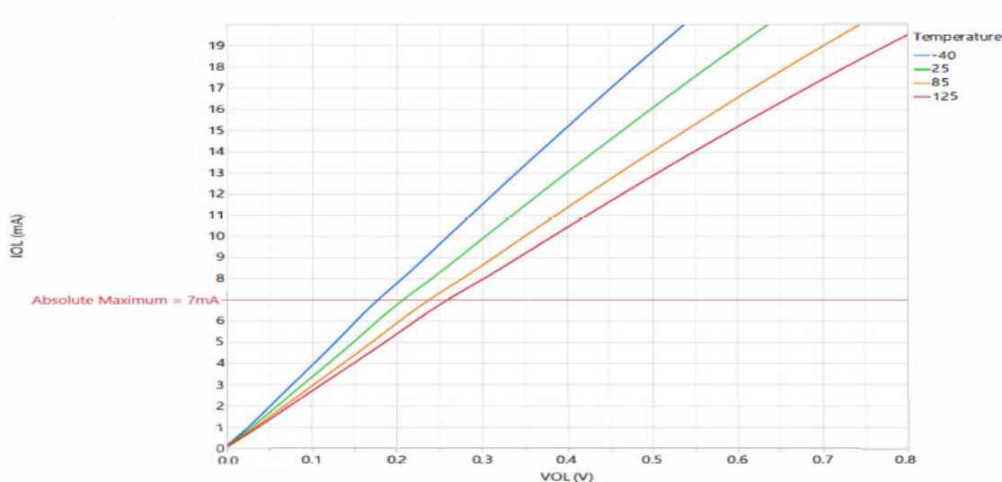
Figure 40-8. IOL vs VOL, 4x Drive Strength I/O on Typical parts with VDDIO = 3.0 V
