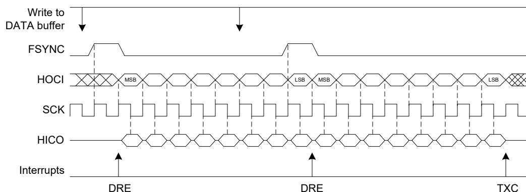
Figure 32-38. FMODE = HOST, FSPOL = HIGH, FSLEN = STROBE, FSER = 0
