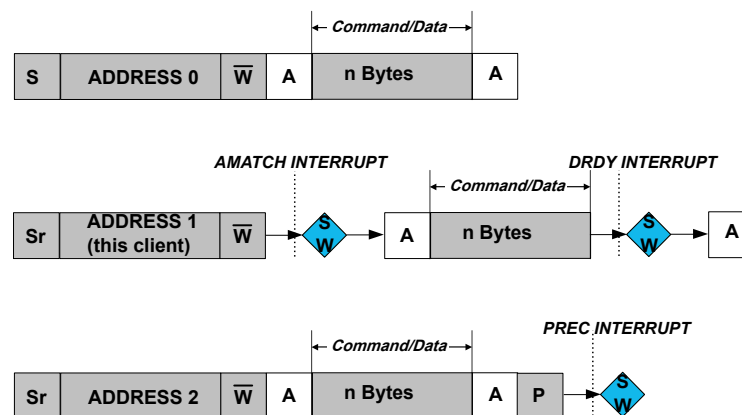
Figure 32-56. PMBus Group Command Example
