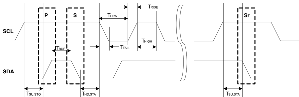
Figure 32-50. SCL Timing
