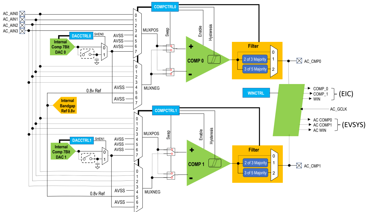
Figure 37-1. Analog Comparator Block Diagram
