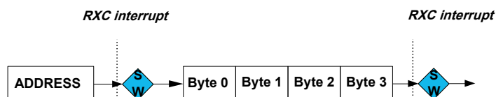
Figure 32-37. 0-bit Extension Client Operation
