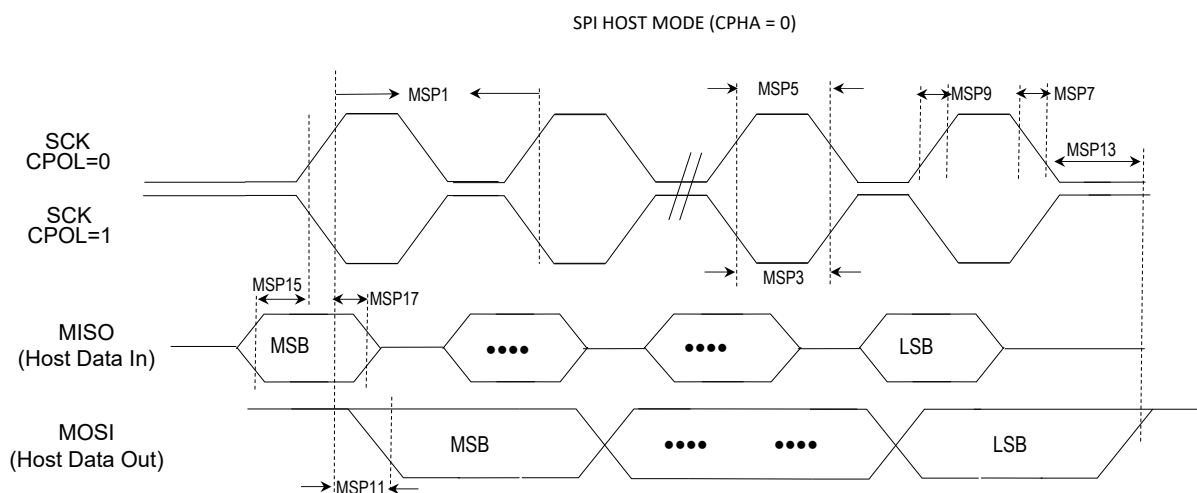
Figure 41-7. SPIx Host Module (CPHA = 0) Timing Diagrams
