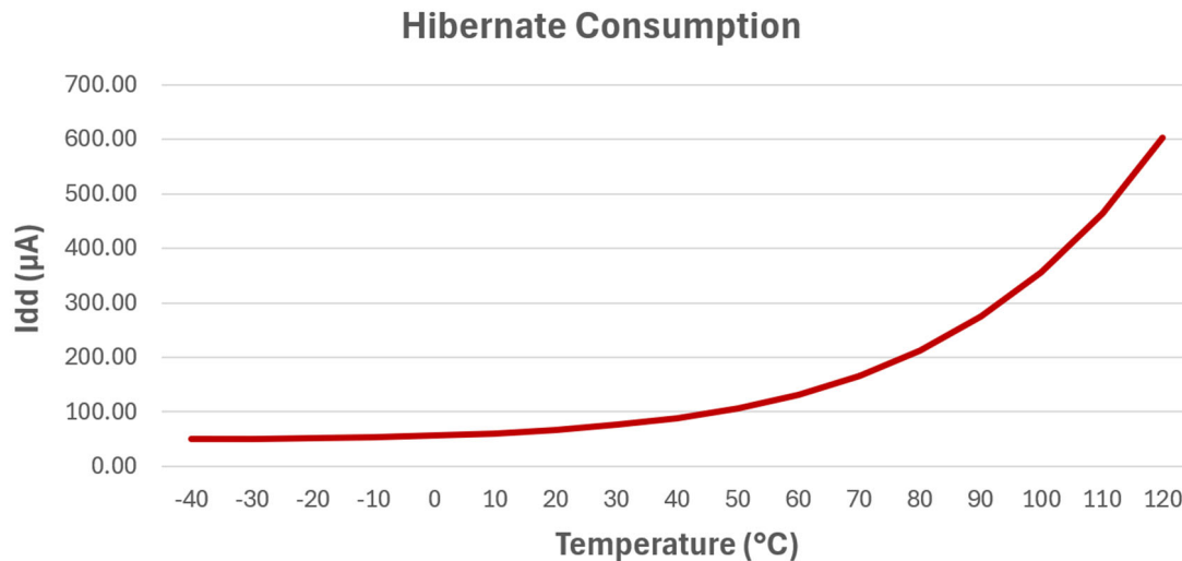
Figure 41-4. Power Consumption over Temperature in Hibernate Mode (Typical values for guidance only, not tested)
