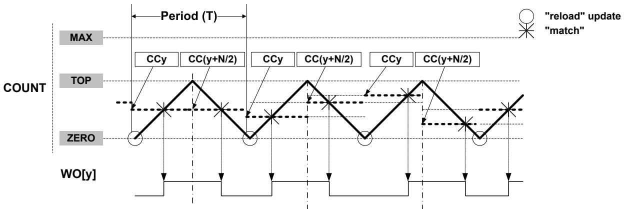
Figure 38-7. Dual-Slope Critical Pulse Width Modulation ( N = \text{CC\_NUM} )
