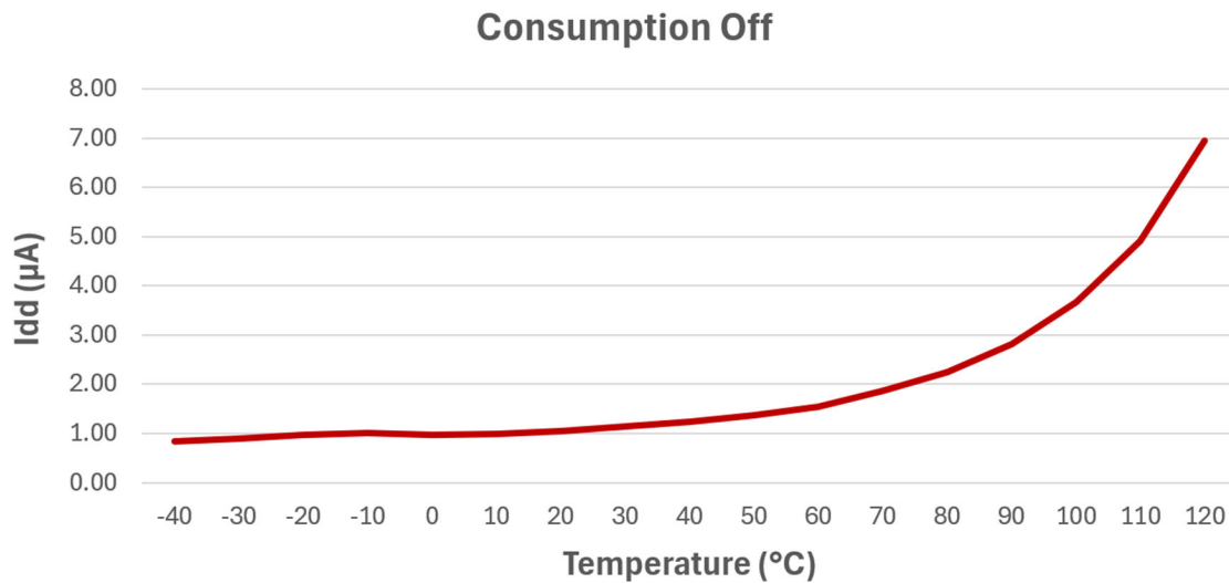
Figure 40-6. Power Consumption over Temperature in Off Mode (Typical values for guidance only, not tested)
