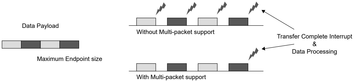
Figure 34-3. Multi-Packet Feature - Reduction of CPU Overhead
