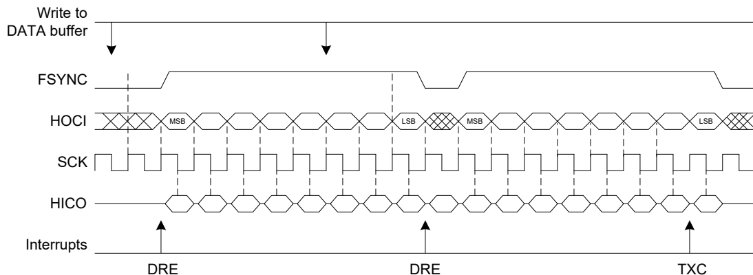
Figure 32-41. FMODE = HOST, FSPOL = HIGH, FSLEN = LEVEL, FSSES = 1
