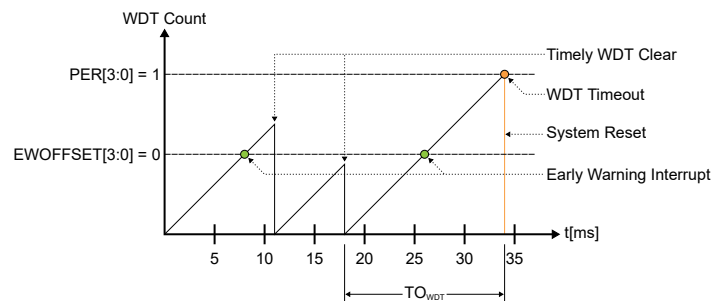
Figure 21-2. Normal-Mode Operation
