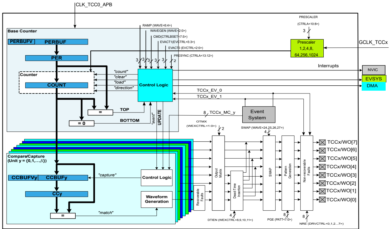
Figure 38-1. Timer/Counter for Control Applications Block Diagram
