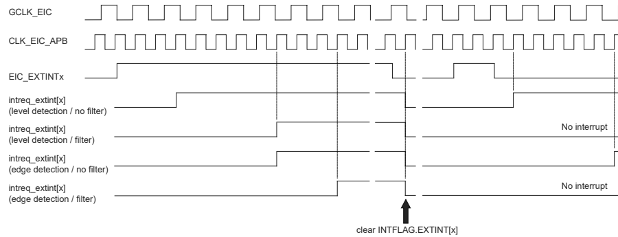
Figure 28-2. Interrupt Detection Latency by Modes (Rising Edge)
