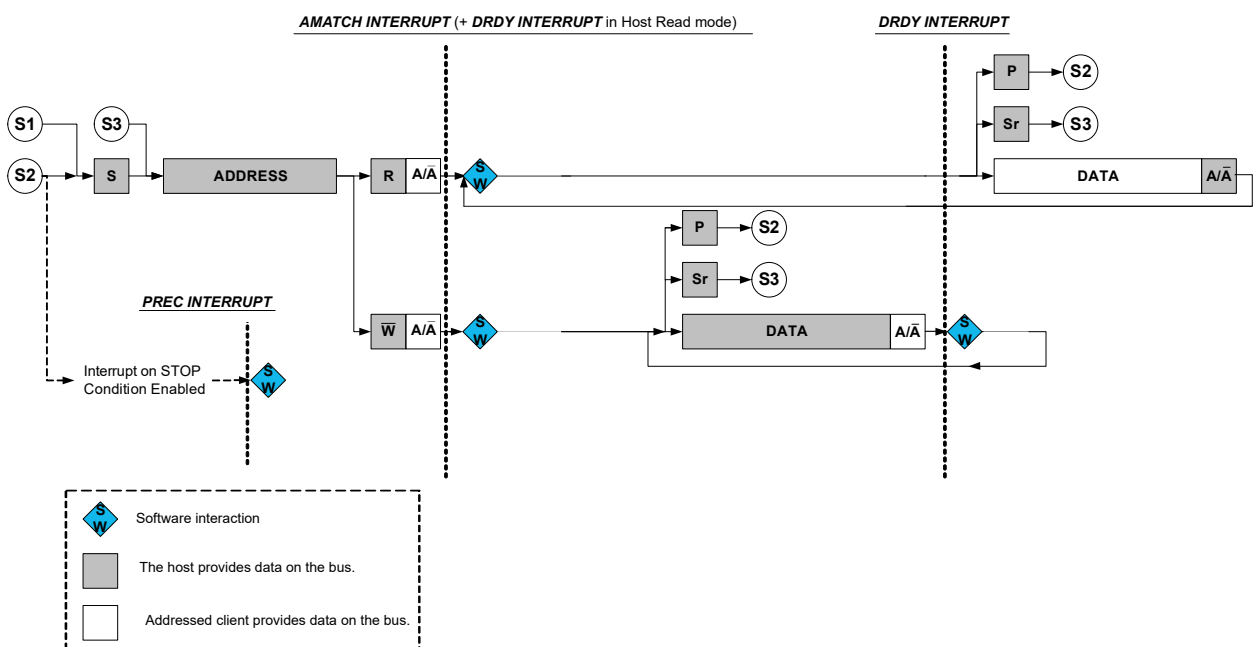
Figure 32-54. I 2 C Client Behavioral Diagram (SCLSM=1)
