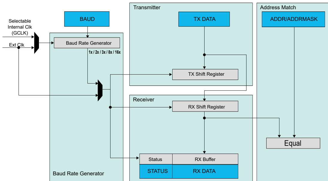
Figure 32-2. SERCOM Serial Engine
