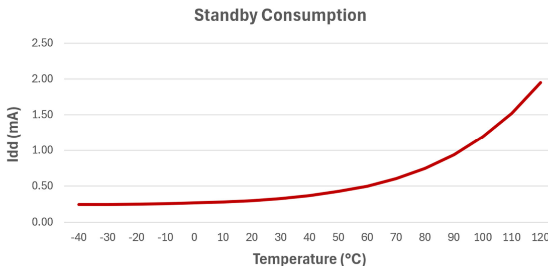
Figure 40-3. Power Consumption over Temperature in Standby Mode (Typical values for guidance only, not tested)
