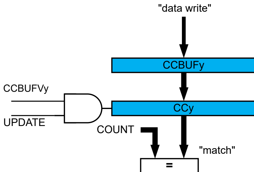
Figure 38-9. Compare Channel Double Buffering
