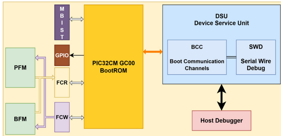
Figure 12-1. PIC32 GC00 Boot ROM Block Diagram
