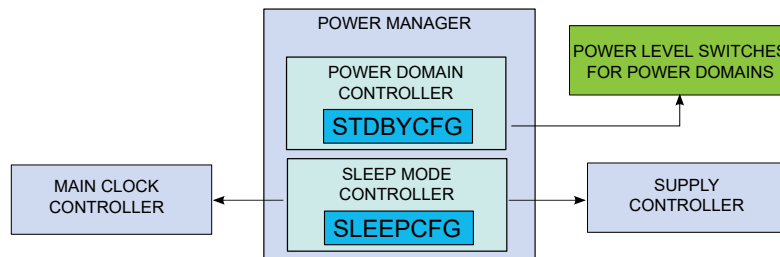
Figure 26-1. Power Manager Block Diagram
