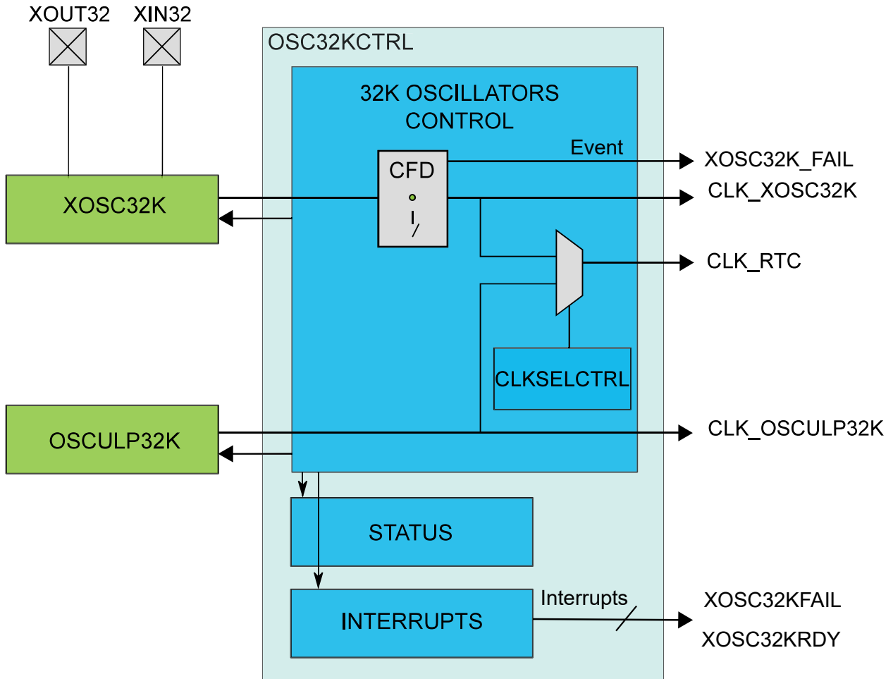
Figure 20-1. OSC32KCTRL Block Diagram
