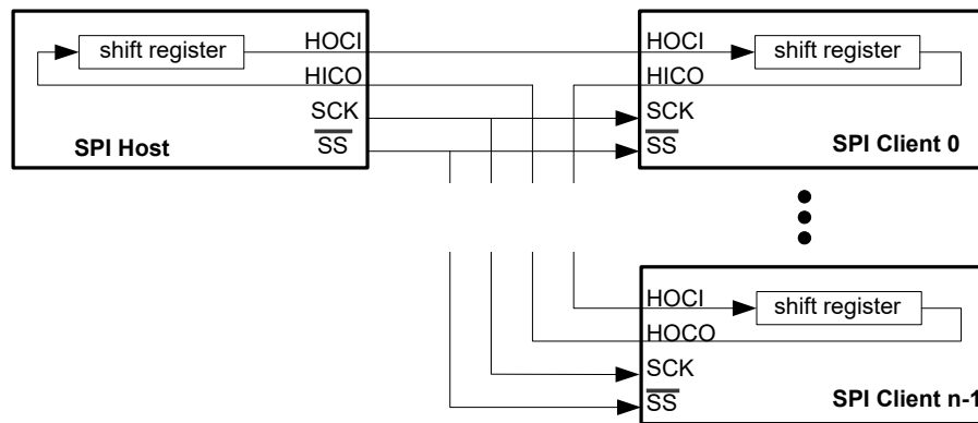
Figure 32-33. Multiple Clients in Series
