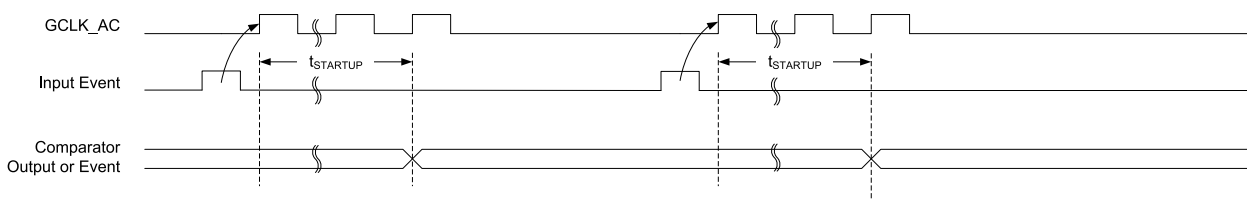
Figure 37-9. Single-Shot SleepWalking
