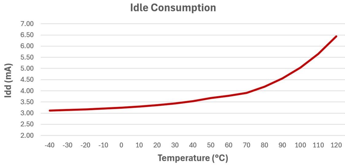
Figure 41-2. Power Consumption over Temperature in IDLE Mode (Typical values for guidance only, not characterized over Process / voltage)
