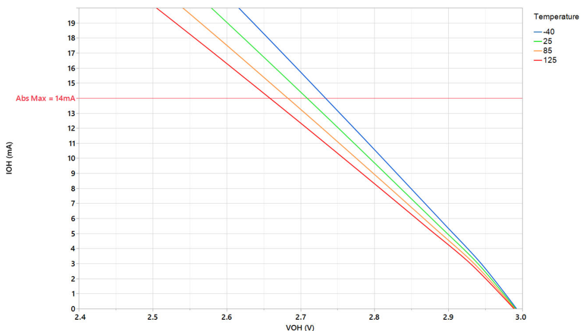
Figure 40-14. IOH vs VOH, 8x Drive Strength I/O on Typical parts with VDDIO = 3.0 V
