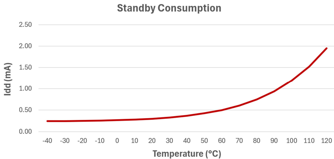
Figure 41-3. Power Consumption over Temperature in Standby Mode (Typical values for guidance only, not tested)
