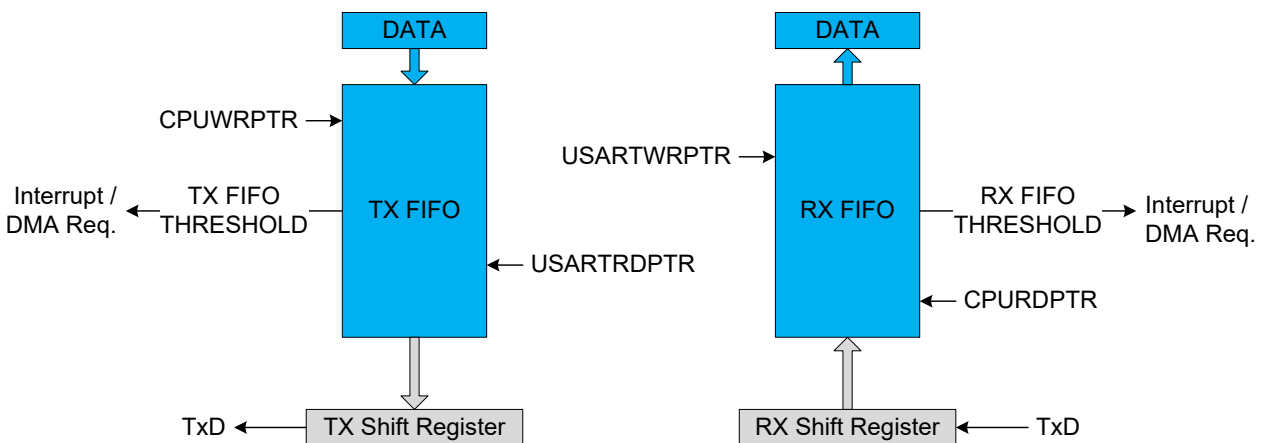
Figure 32-27. FIFO Overview
