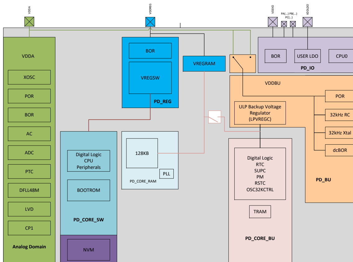
Figure 7-1. Power Domain Block Diagram
