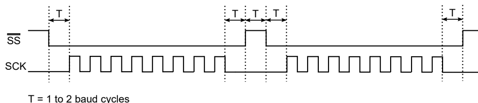
Figure 32-34. Hardware Controlled \overline{SS}
