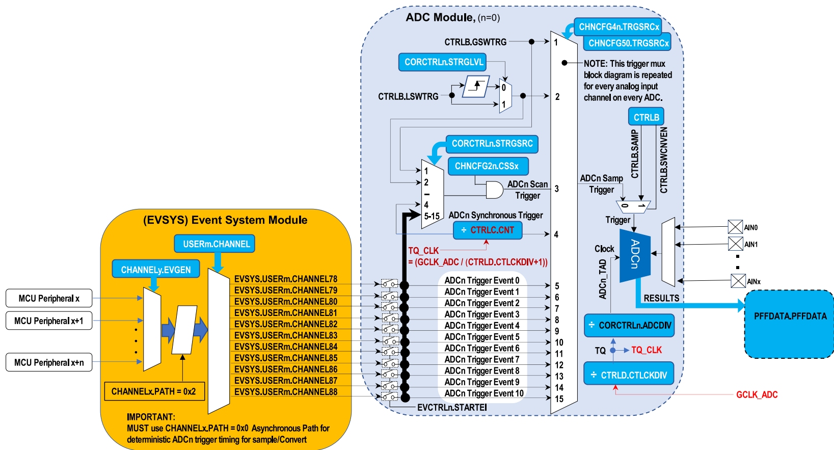
Figure 36-2. ADC Trigger Block Diagram
