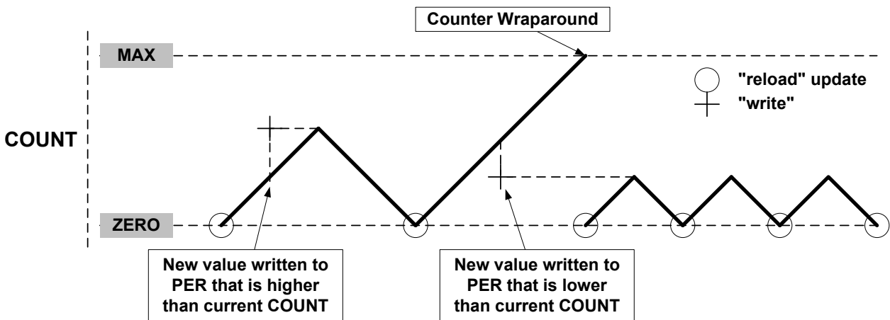
Figure 38-12. Unbuffered Dual-Slope Operation
