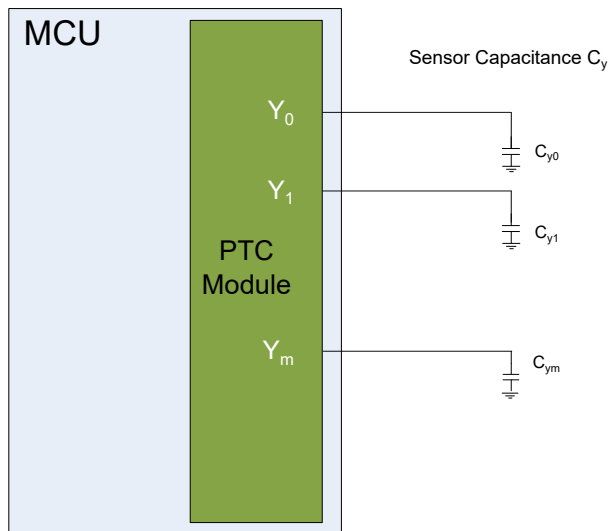
Figure 39-4. Self-Capacitance Sensor Arrangement
