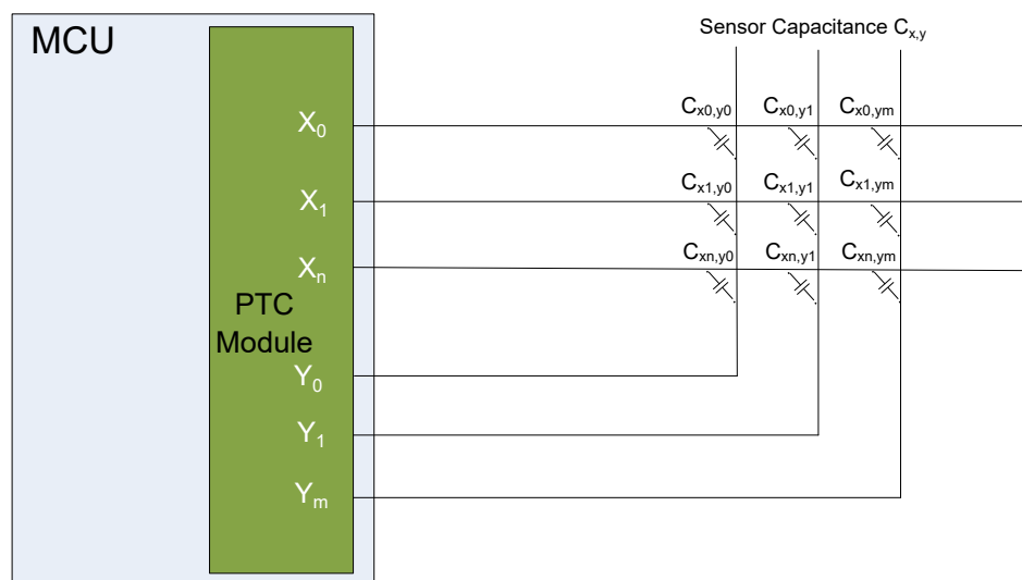
Figure 39-3. Mutual Capacitance Sensor Arrangement
