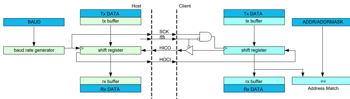
Figure 32-28. Full-Duplex SPI Host Client Interconnection
