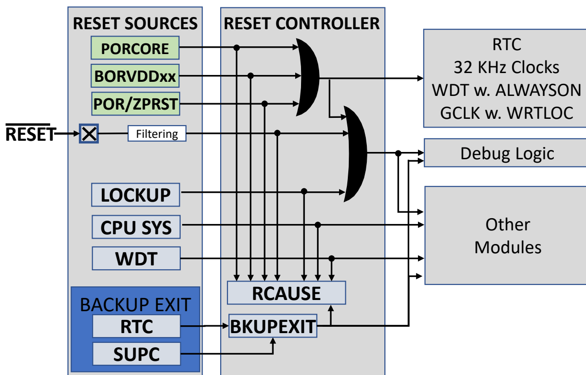
Figure 27-1. Reset Controller Block Diagram
