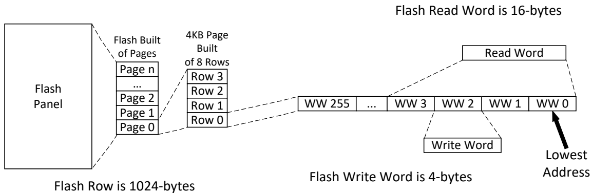
Figure 29-1. Flash Module Construction
