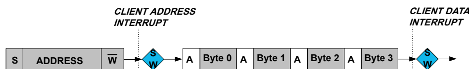
Figure 32-59. 32-bit Extension Client Operation
