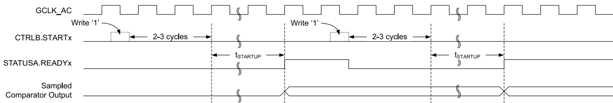
Figure 37-3. Single-Shot Example
