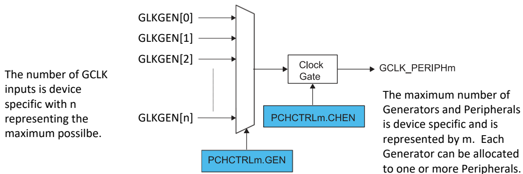
Figure 18-4. Peripheral Clock
