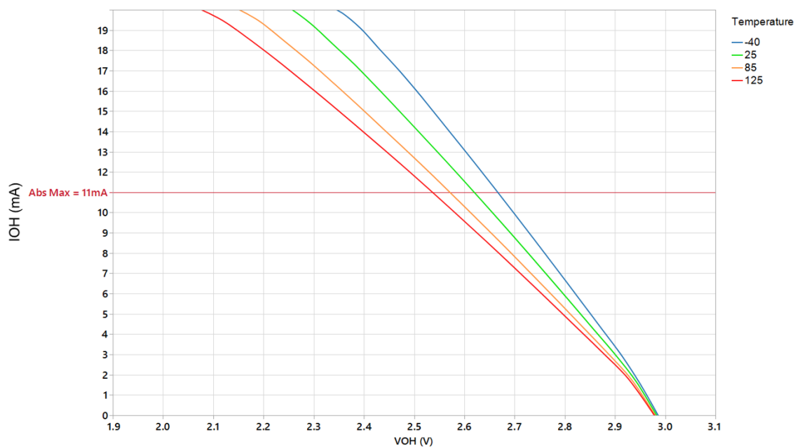
Figure 40-12. IOH vs VOH, 4x Drive Strength I/O on Typical parts with VDDIO = 3.0 V
