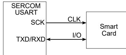
Figure 32-20. Connection of a Smart Card to the SERCOM USART
