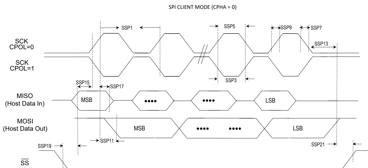
Figure 41-9. SPIx Client Module (CPHA = 0) Timing Diagrams
