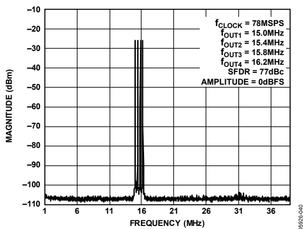
Figure 26. Four-Tone SFDR
