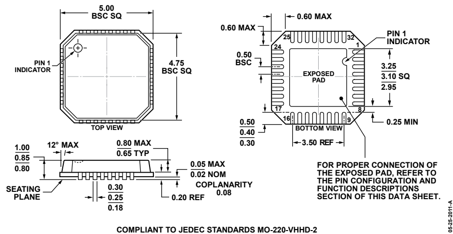
COMPLIANT TO JEDEC STANDARDS MO-220-VHHD-2 Figure 91. 32-Lead Lead Frame Chip Scale Package [LFCSP_VQ] 5 mm × 5 mm, Very Thin Quad (CP-32-2) Dimensions shown in millimeters
