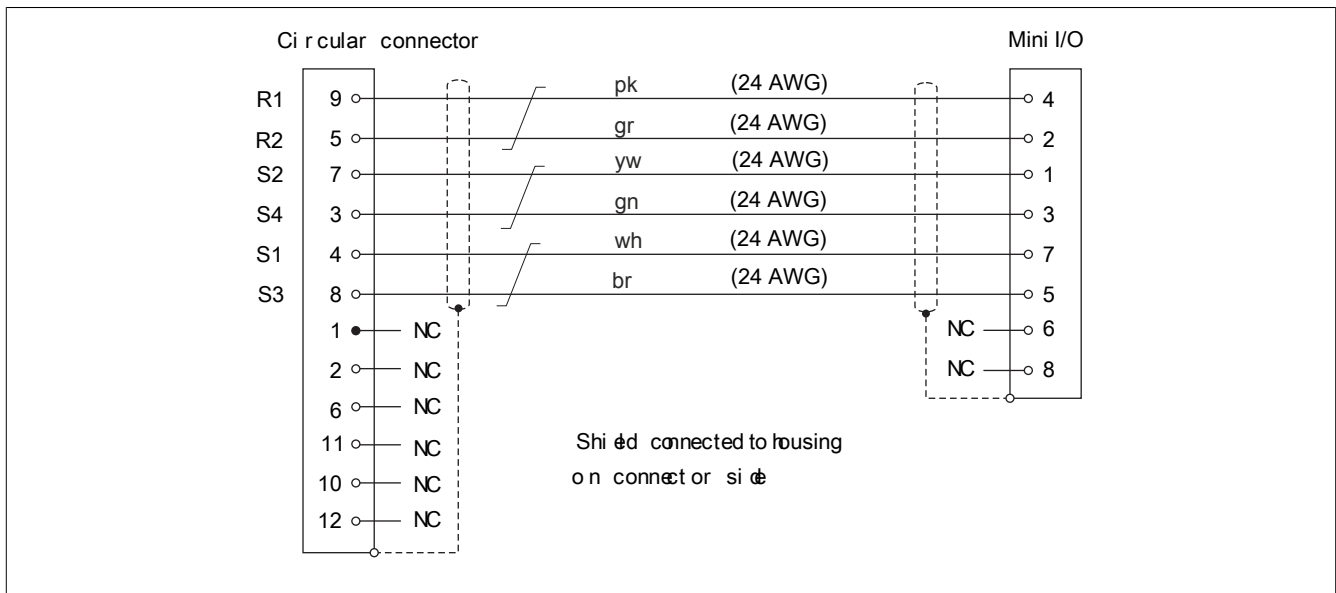
Figure 1: 8ECR resolver cables - Cable diagram
