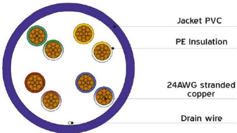
Technical Drawing:
