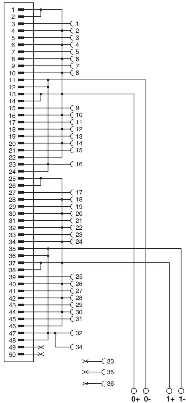
Circuit diagram
