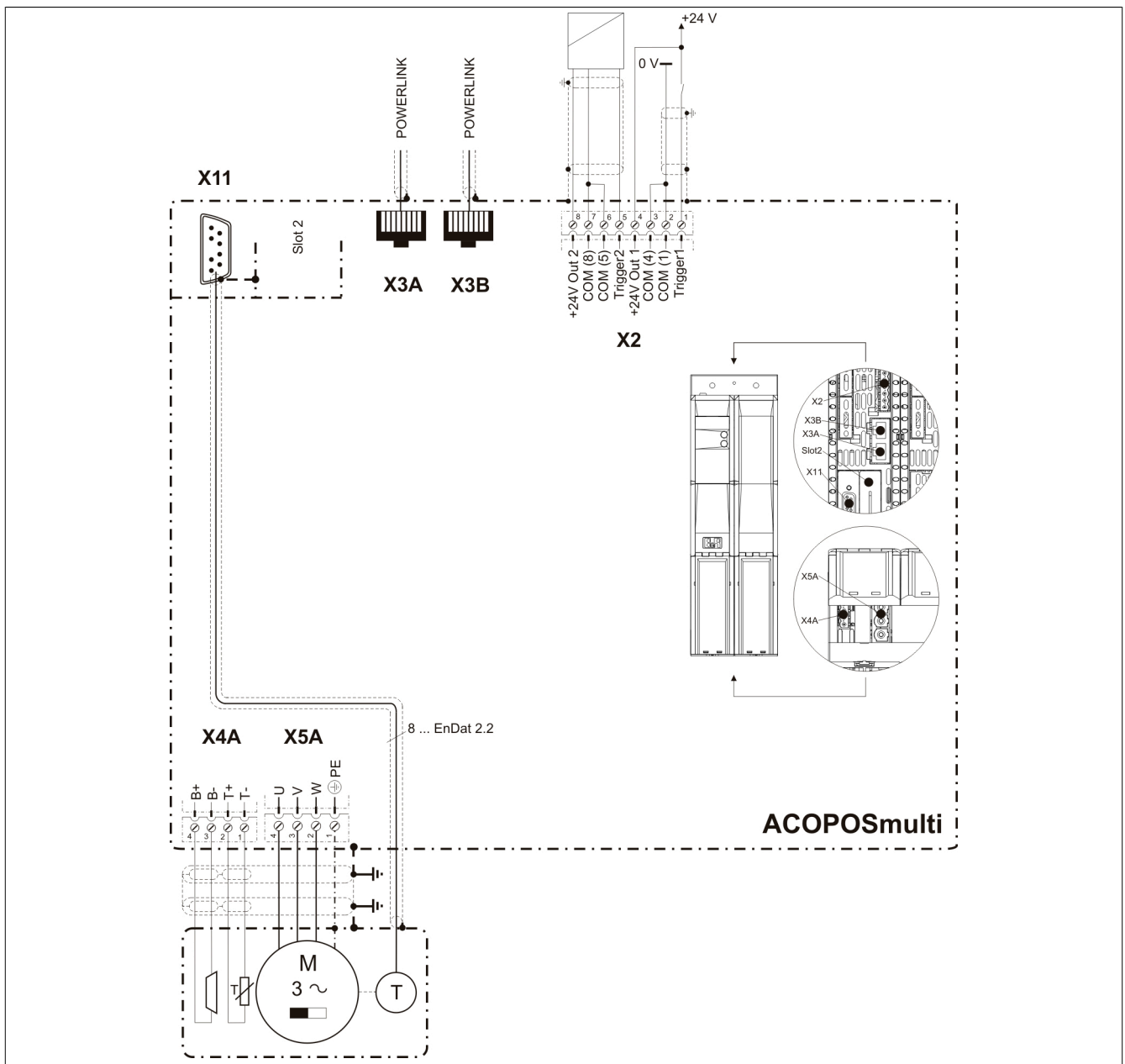
Figure 6: Pinout overview
