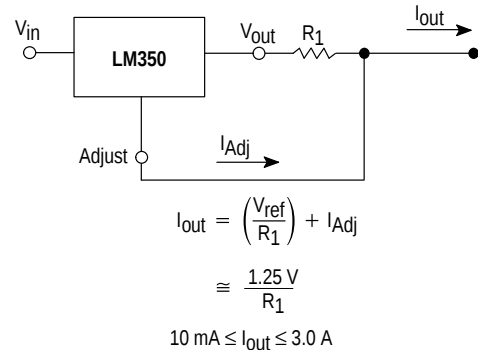
Figure 23. Current Regulator
