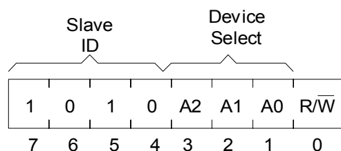
Figure 4. Slave Address
