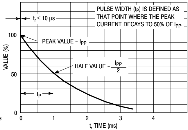
Figure 2. Pulse Waveform
