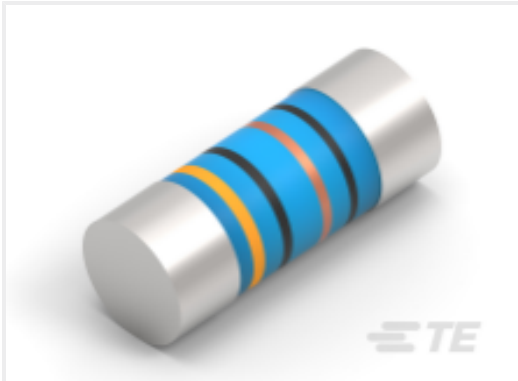
TE Part #3-2176315-6 MELF SMA_A 82K 0.1% 15PPM 0204 0.4W
