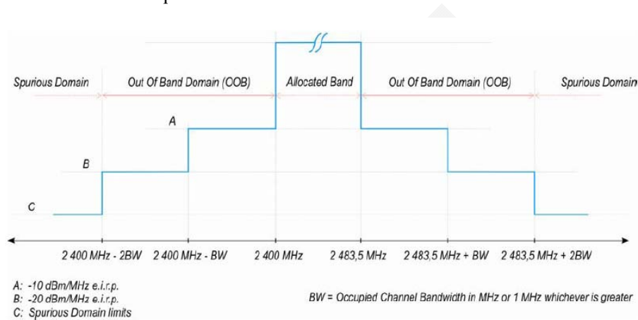
Figure 1: Transmit mask
