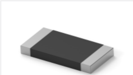
TE Part #2-2176421-5 TLRP 2512 2.0W R040 1% 25PPM 4K RL
