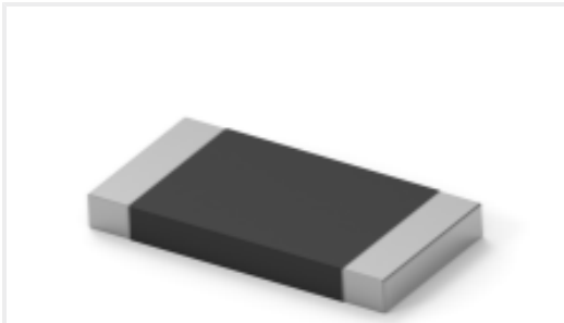
TE Part #3-2176422-8 TLRP 2512 3.0W R080 1% 25PPM 4K RL
