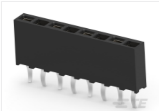
TE Part # 215297-8 8P HV100 REC CON. TE, 7.0MM
