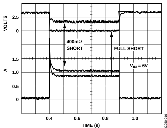
Figure 16. Short-Circuit Current
