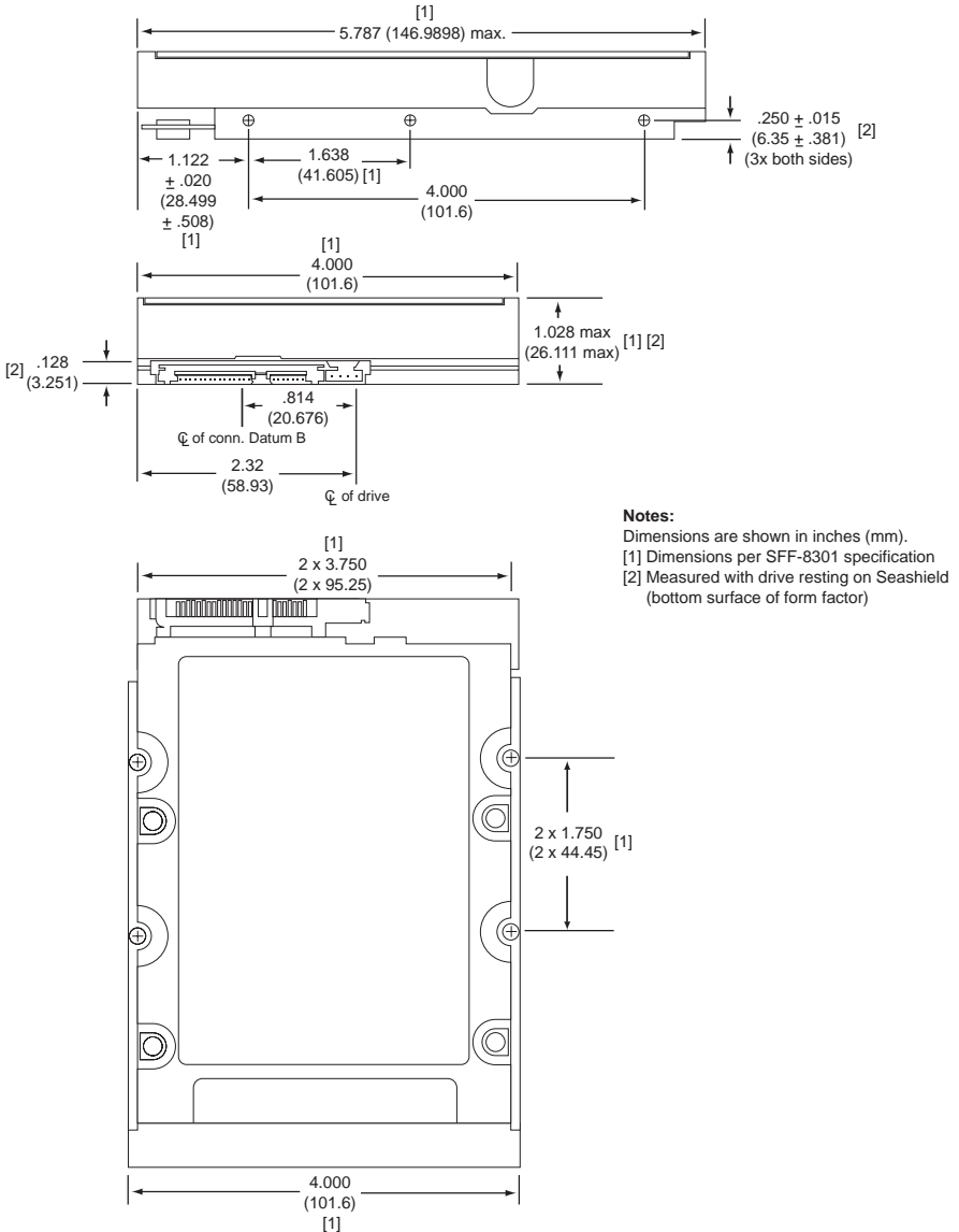
Figure 7. Mounting dimensions—top, side and end view
