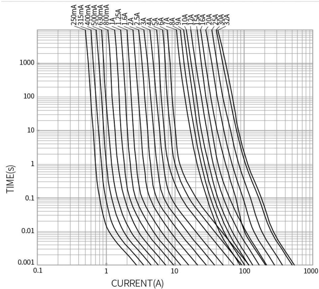
AVERAGE I-T CHARACTERISTICS CURVE (FOR REFERENCE ONLY)
