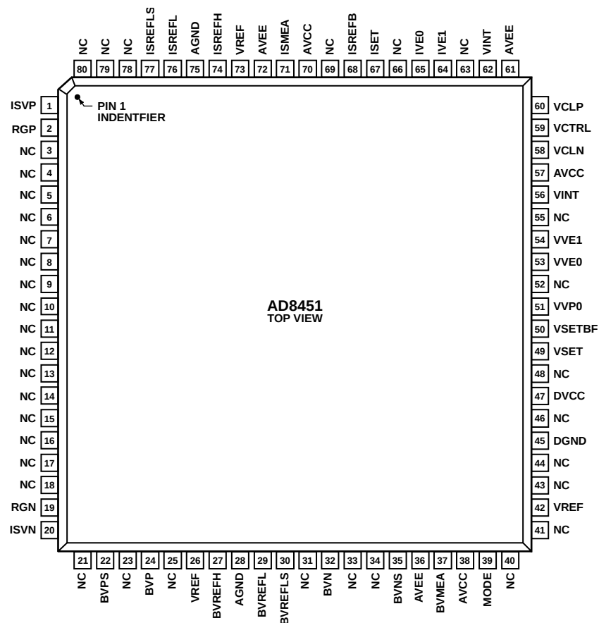
Figure 2. Pin Configuration
