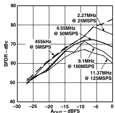
Figure 27. Single-Tone SFDR vs. A_{OUT} @ f_{OUT} = f_{CLOCK}/11
