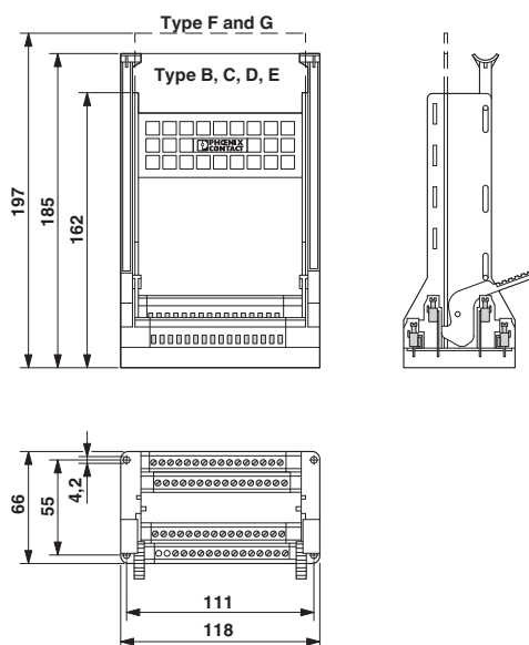
Dimensioned drawing
