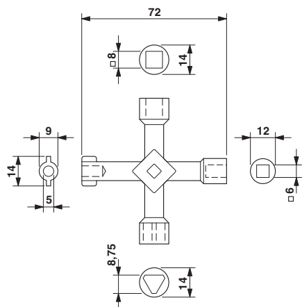
Dimensional drawing
