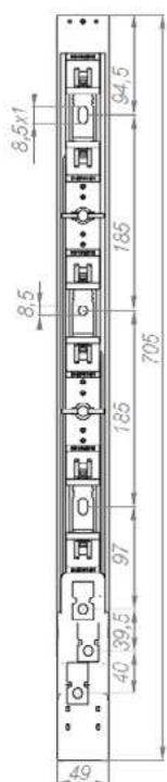
M8 Screws
