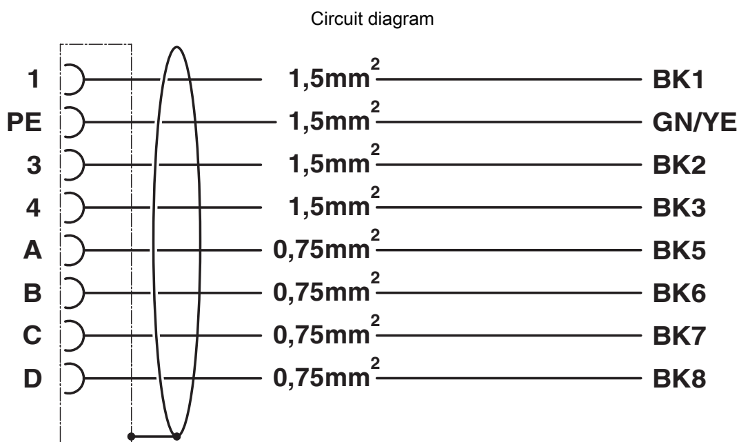
Contact assignment of M23 plugs/sockets
