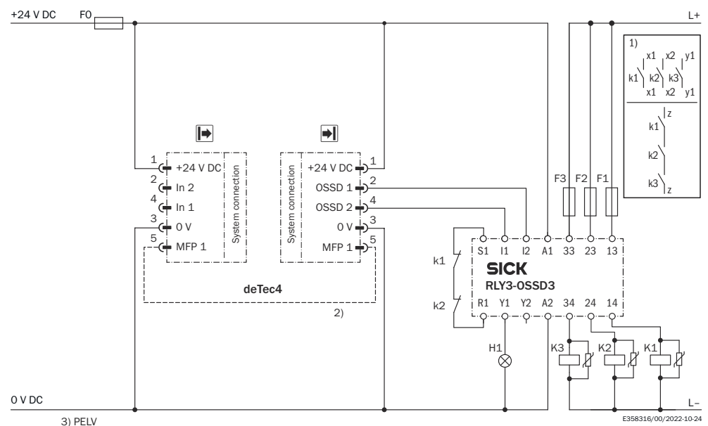
Figure 6: ReLy OSSD3 connection diagram, without restart interlock, with external device monitoring (EDM)
