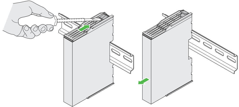
Figure 9: Disassembly
