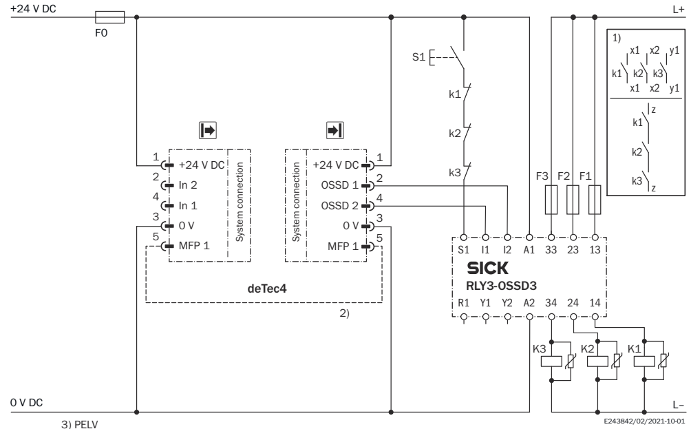
Figure 5: ReLy OSSD3 connection diagram, with restart interlock and external device monitoring (EDM)
