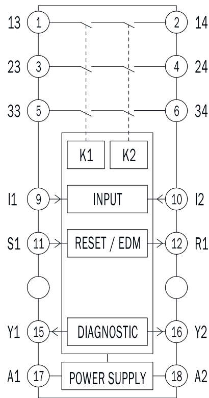
Figure 16: Internal circuitry
