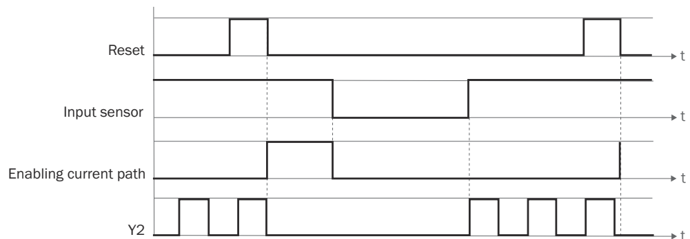
Figure 4: Sequence/timing diagram
