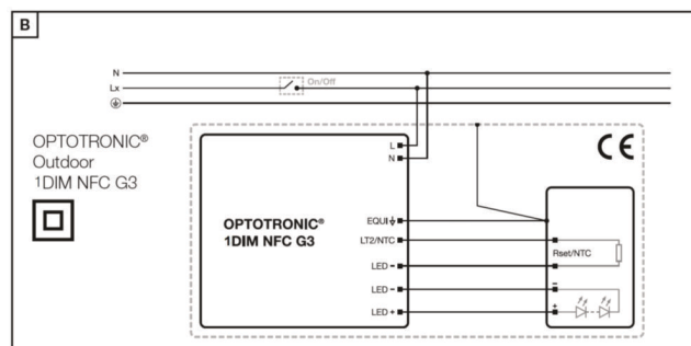
OT 1DIM G3 Wiring diagram II
