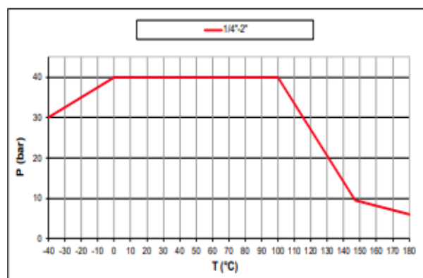
PRESSURE-TEMPERATURE CHART
