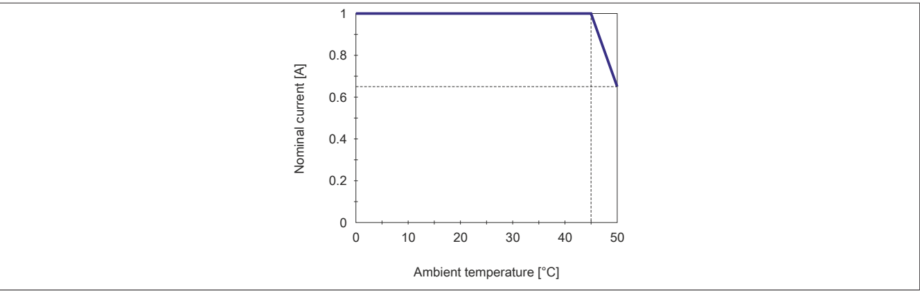
Figure 4: Current derating
