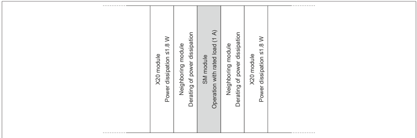
Figure 1: Operating the SM module over the entire temperature range at 1.0 A rated current
