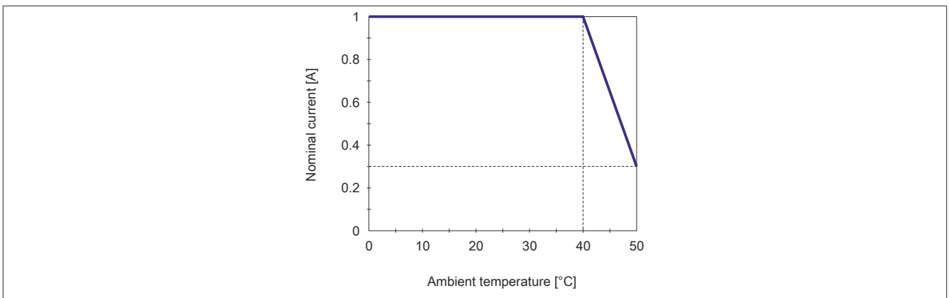
Figure 6: Current derating
