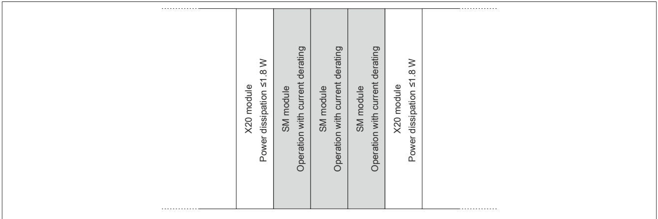
Figure 5: Operating three or more SM modules in a cluster
