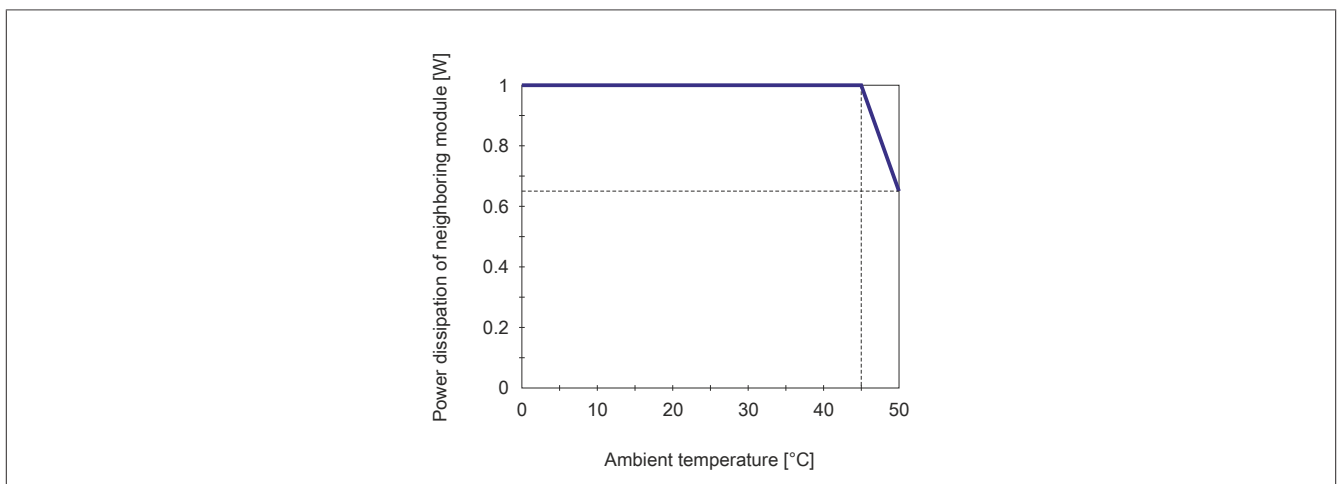
Figure 2: Power loss derating for directly neighboring modules
