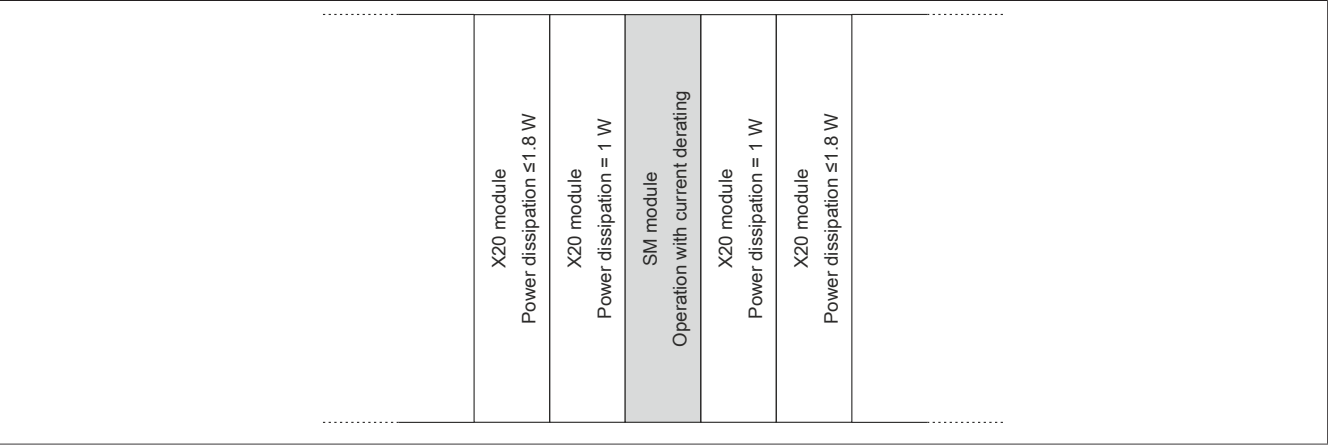
Figure 3: Neighboring modules to the SM module have a power loss of 1.0 W
