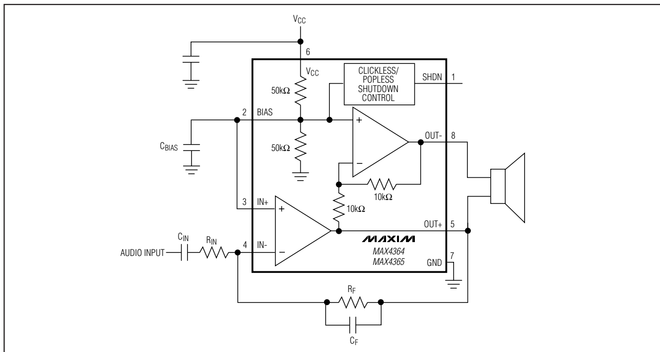
Figure 2. High-Gain Configuration
