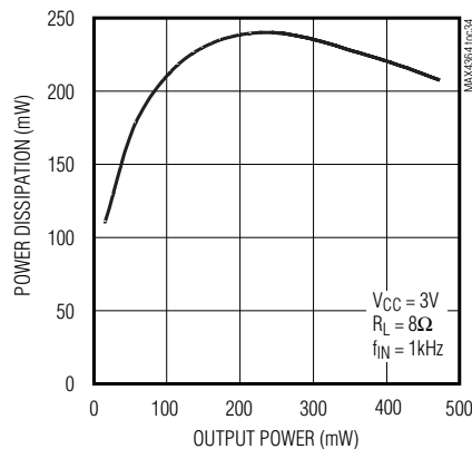
MAX4365 POWER DISSIPATION vs. OUTPUT POWER
