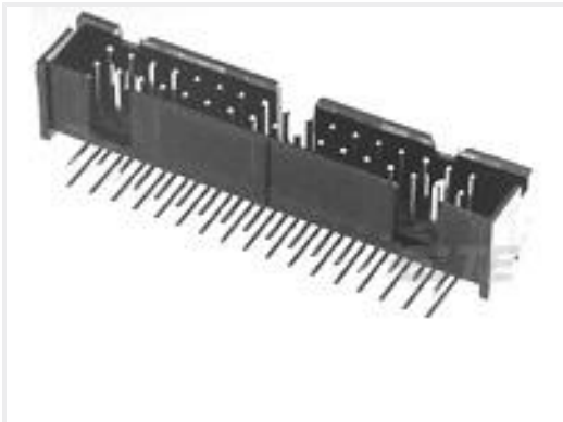
TE Part #5103310-7 A/L LOW PRO HDR 34P RA BLACK
