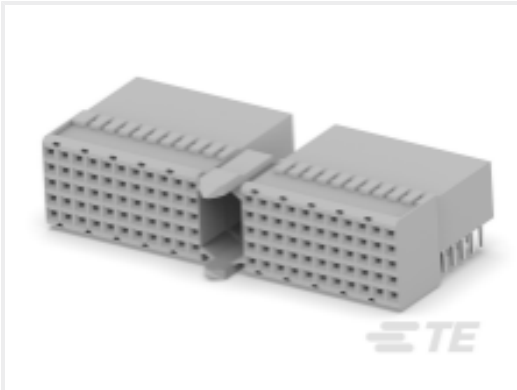
TE Part #3-5100147-0 Z-PACK,TYPE A, RA REC.110P
