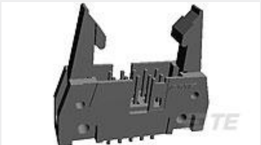
TE Part #1-5102321-2 A/L UNIV HDR 64P VERT LAT
