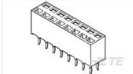
TE Part #1-215307-0 2X10P HV100 REC CON. TE, 7.0MM
