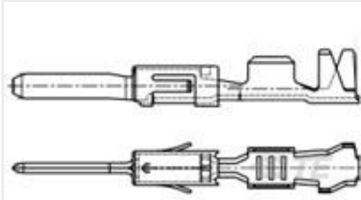
TE Part #963902-1 TAB A 1.6x0.6 CONTACT CS SWS Sn
