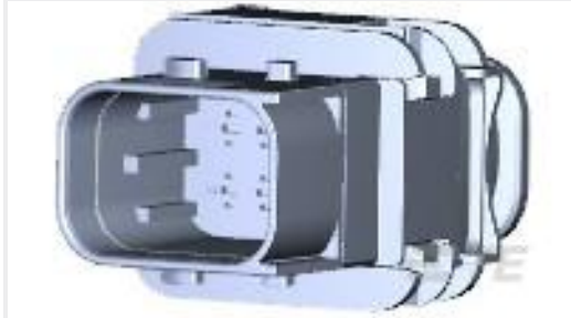
TE Part #1-1564512-1 8POS,TAB 1.6X0.6,TAB HSG,ASSY
