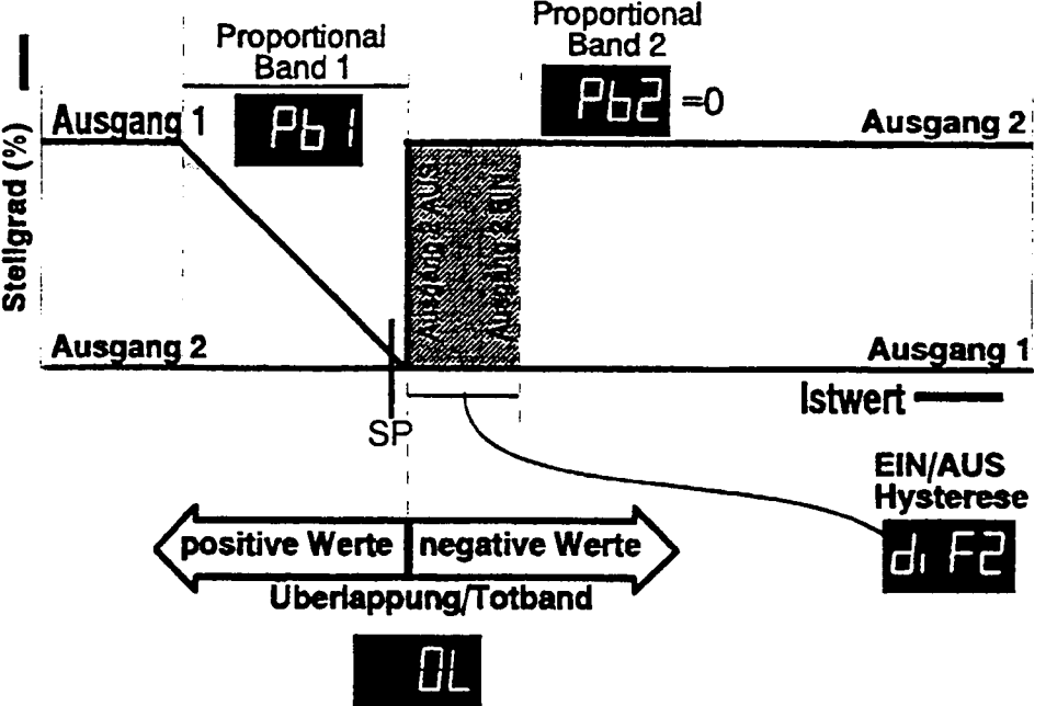
Abb.: 4-2 Proportionalband & Totband/Überlappung
