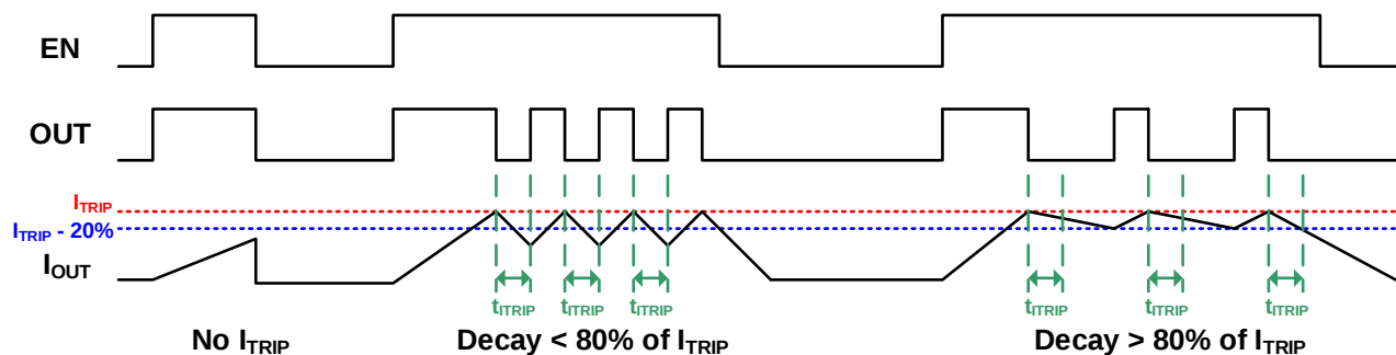
Figure 2: Current Regulation
