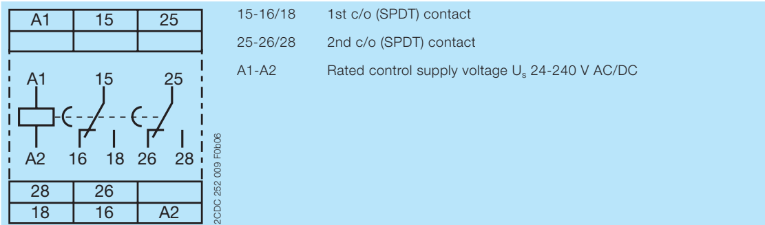
Connection diagram
