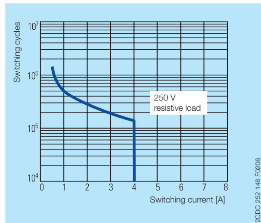
Contact lifetime
