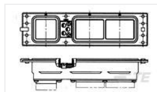
TE Part #1663556-1 RECPT ASSY, SZ 2, ARINC 600
