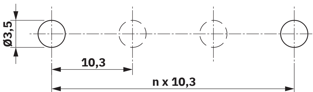
Dimensional drawing
